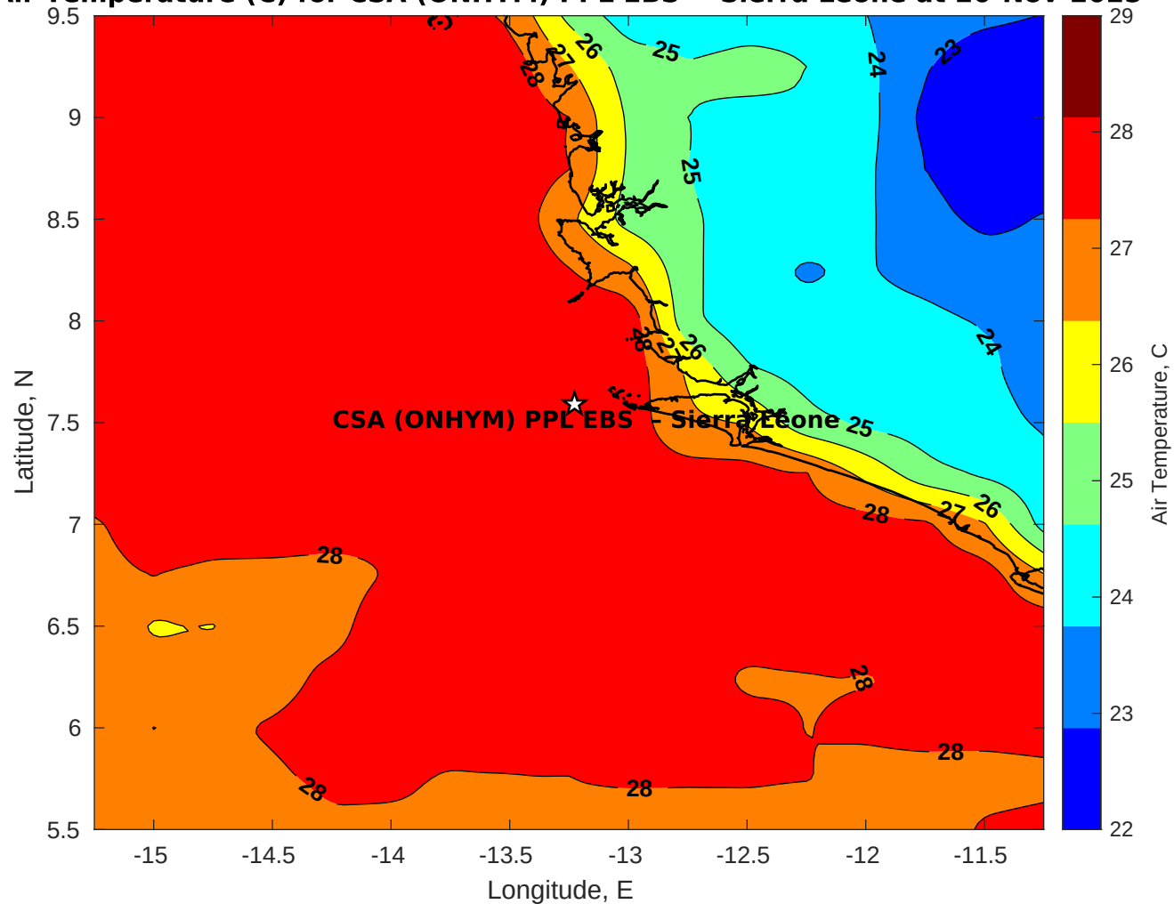
Air Temperature (C) for CSA (ONHYM) PPL EBS - Sierra Leone at 20-Nov-2025
