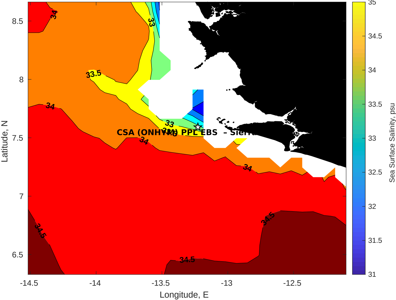
Surface Salinity for CSA (ONHYM) PPL EBS - Sierra Leone at 19-Nov-2025 00:00:00
