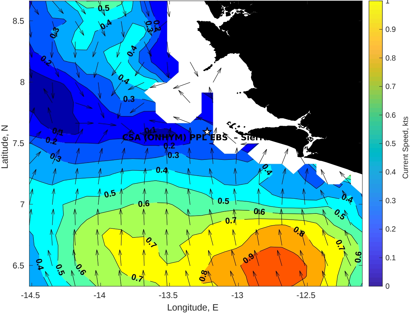
Surface Currents for CSA (ONHYM) PPL EBS - Sierra Leone at 19-Nov-2025 00:00:00
