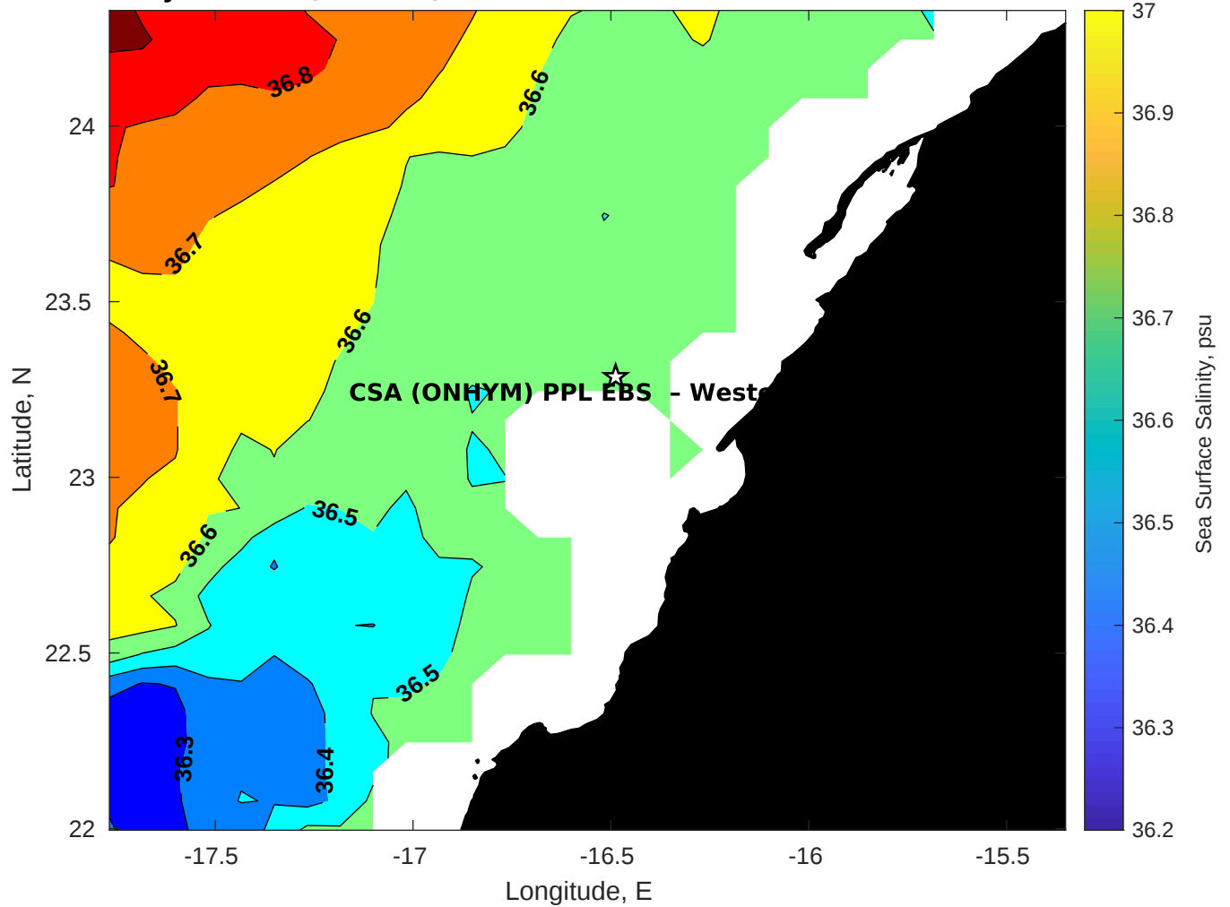
Surface Salinity for CSA (ONHYM) PPL EBS - Western Sahara at 19-Nov-2025 00:00:00
