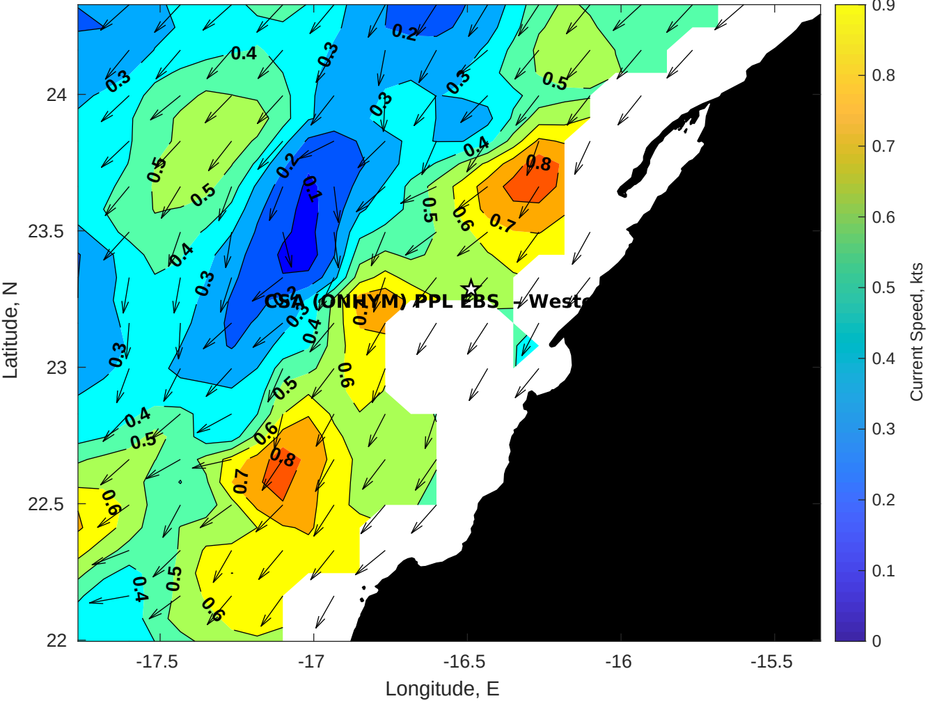
Surface Currents for CSA (ONHYM) PPL EBS - Western Sahara at 19-Nov-2025 00:00:00
