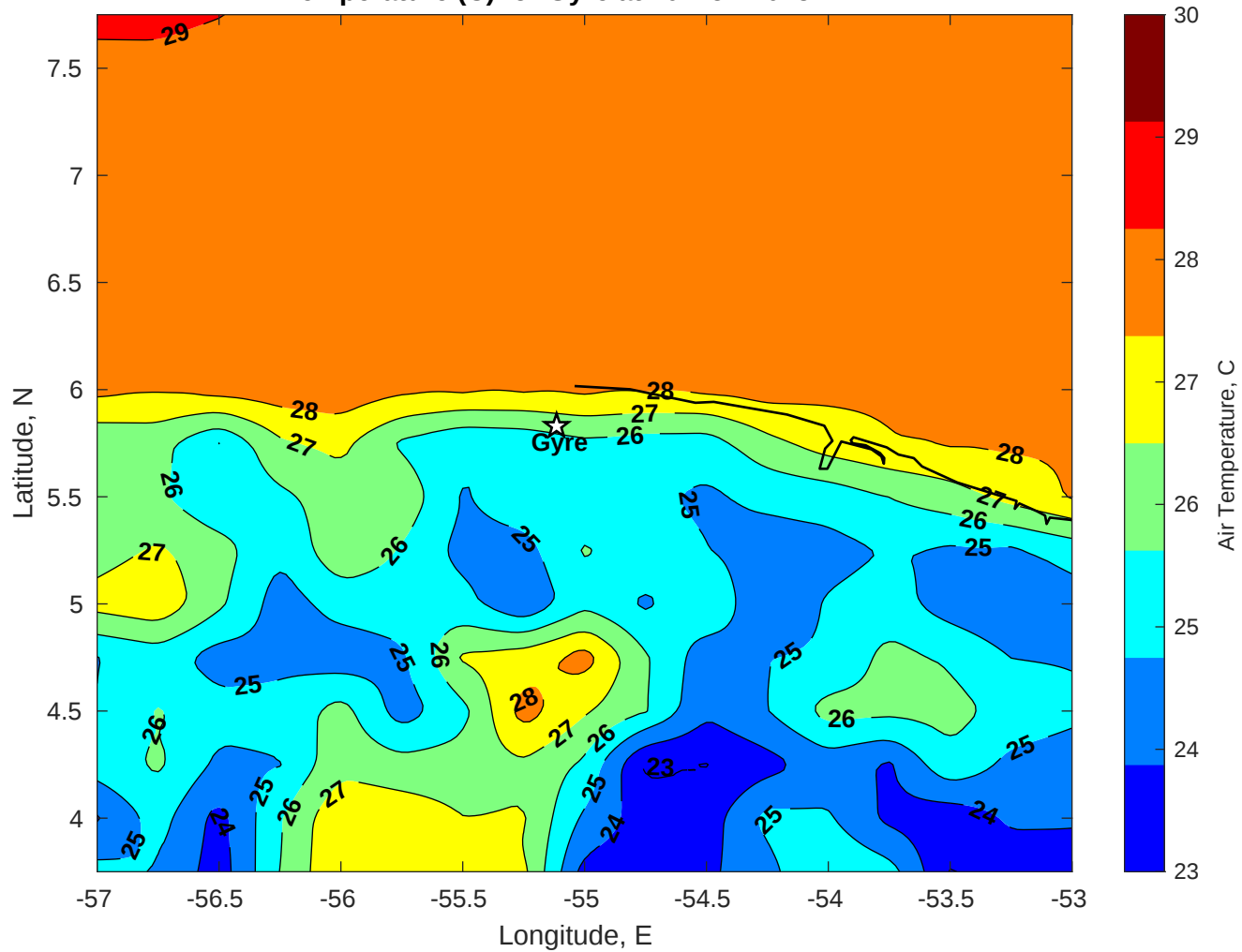
Air Temperature (C) for Gyre at 20-Nov-2025
