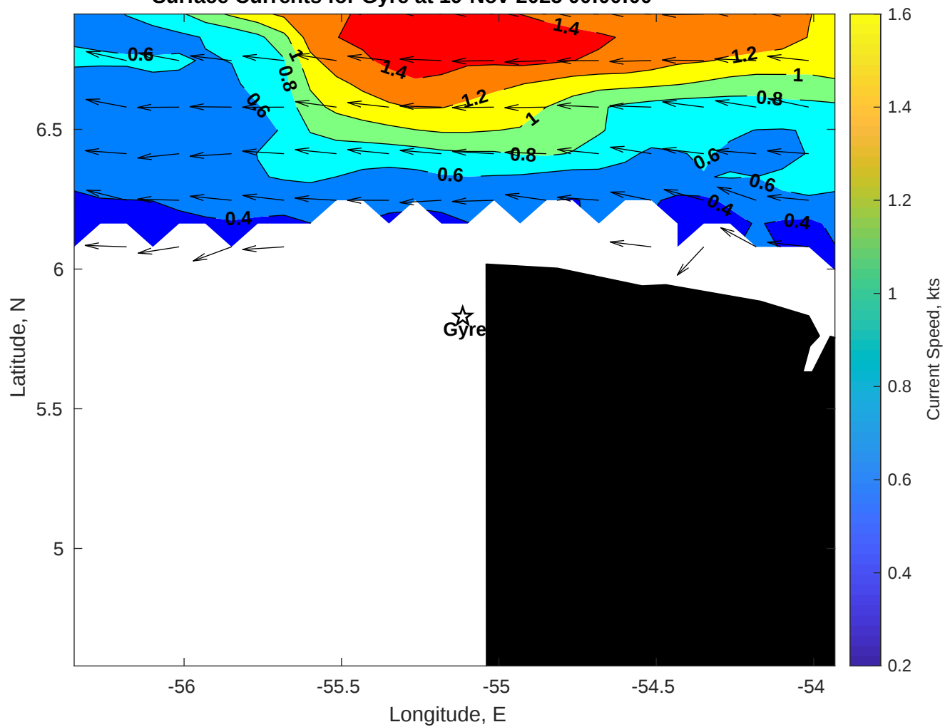
Surface Currents for Gyre at 19-Nov-2025 00:00:00
