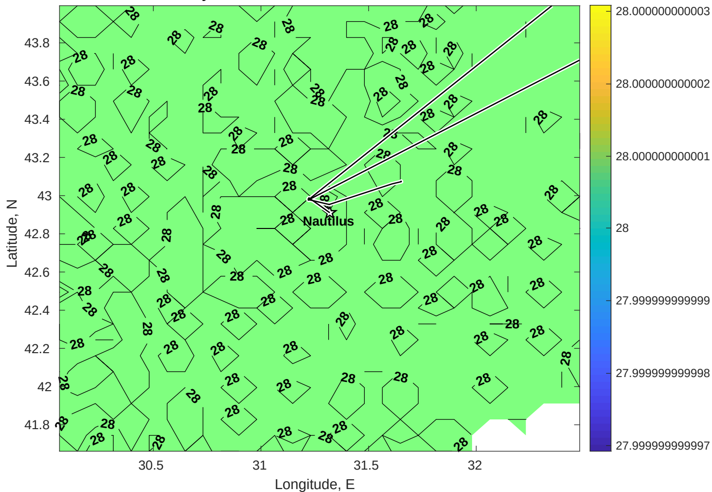
Surface Salinity for Nautilus at 19-Nov-2025 00:00:00
