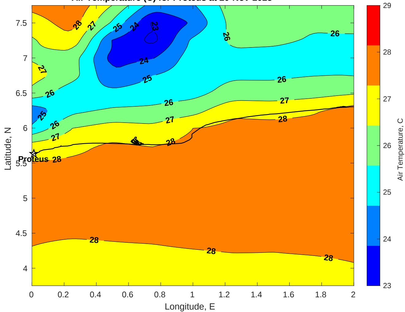
Air Temperature (C) for Proteus at 20-Nov-2025
