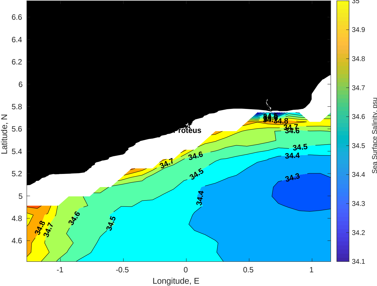
Surface Salinity for Proteus at 19-Nov-2025 00:00:00
