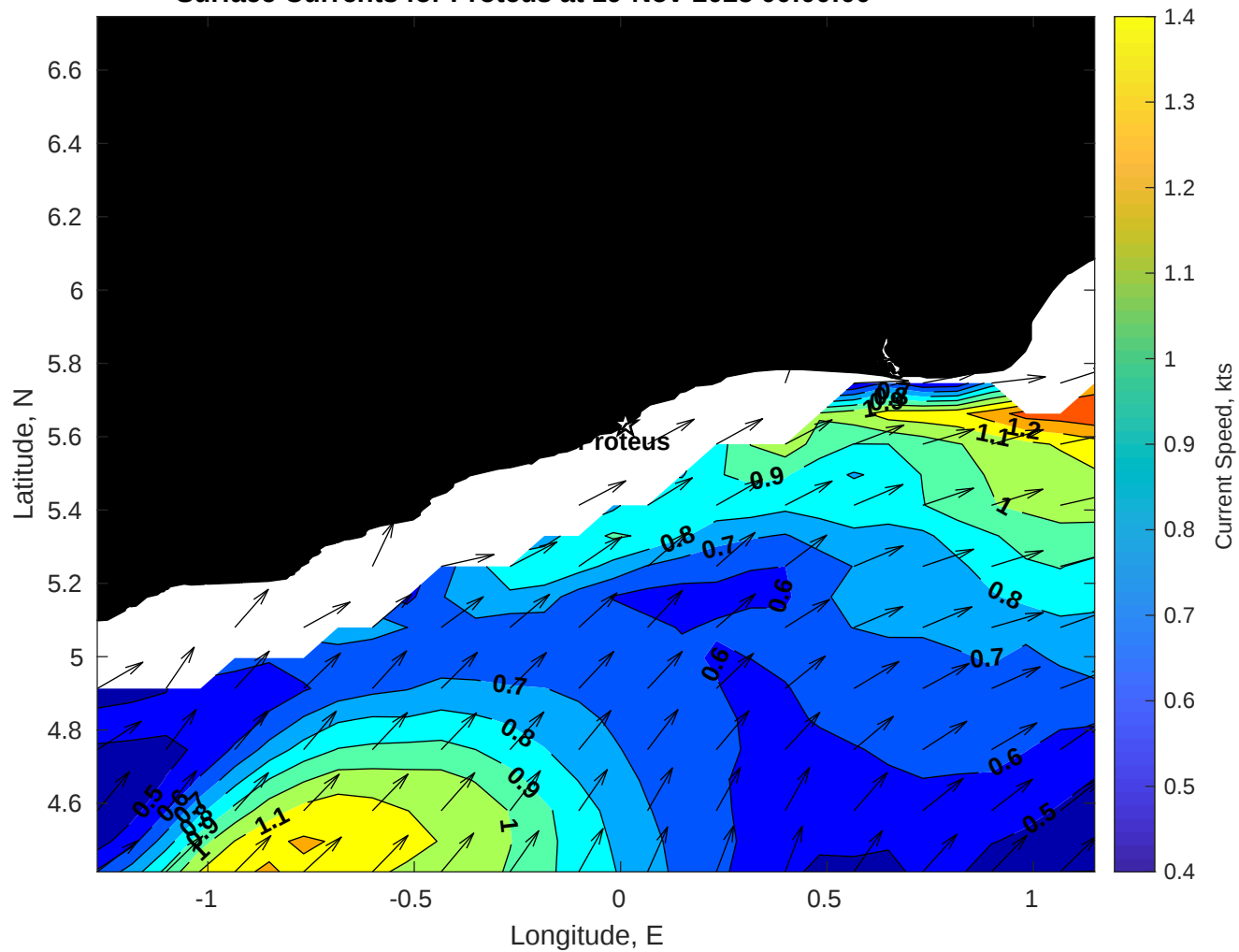
Surface Currents for Proteus at 19-Nov-2025 00:00:00
