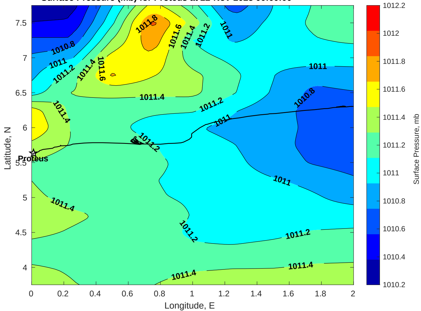
Surface Pressure (mb) for Proteus at 22-Nov-2025 00:00:00
