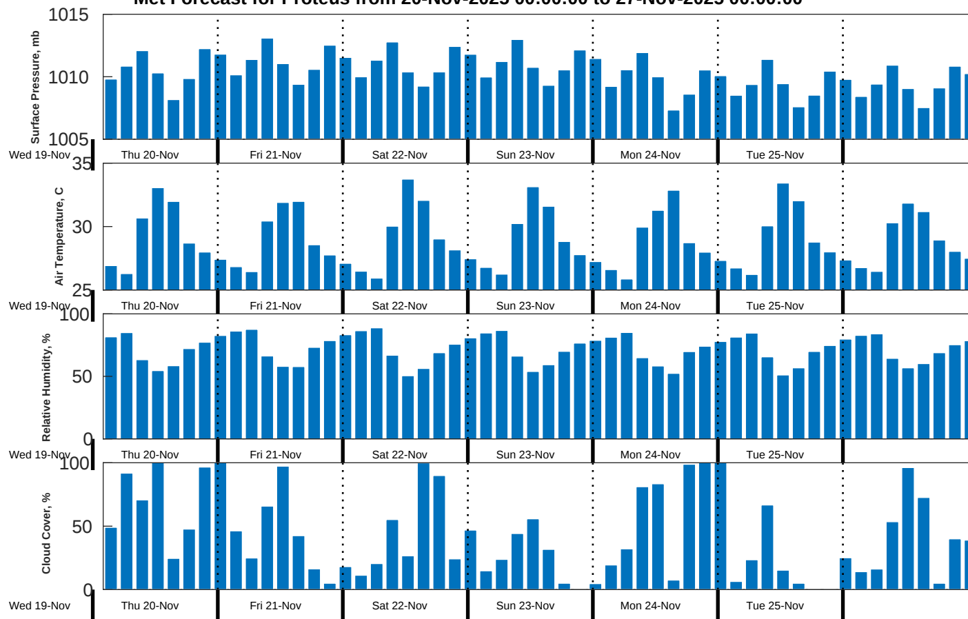
Met Forecast for Proteus from 20-Nov-2025 00:00:00 to 27-Nov-2025 00:00:00
