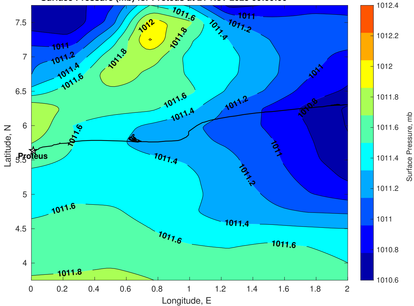
Surface Pressure (mb) for Proteus at 21-Nov-2025 00:00:00
