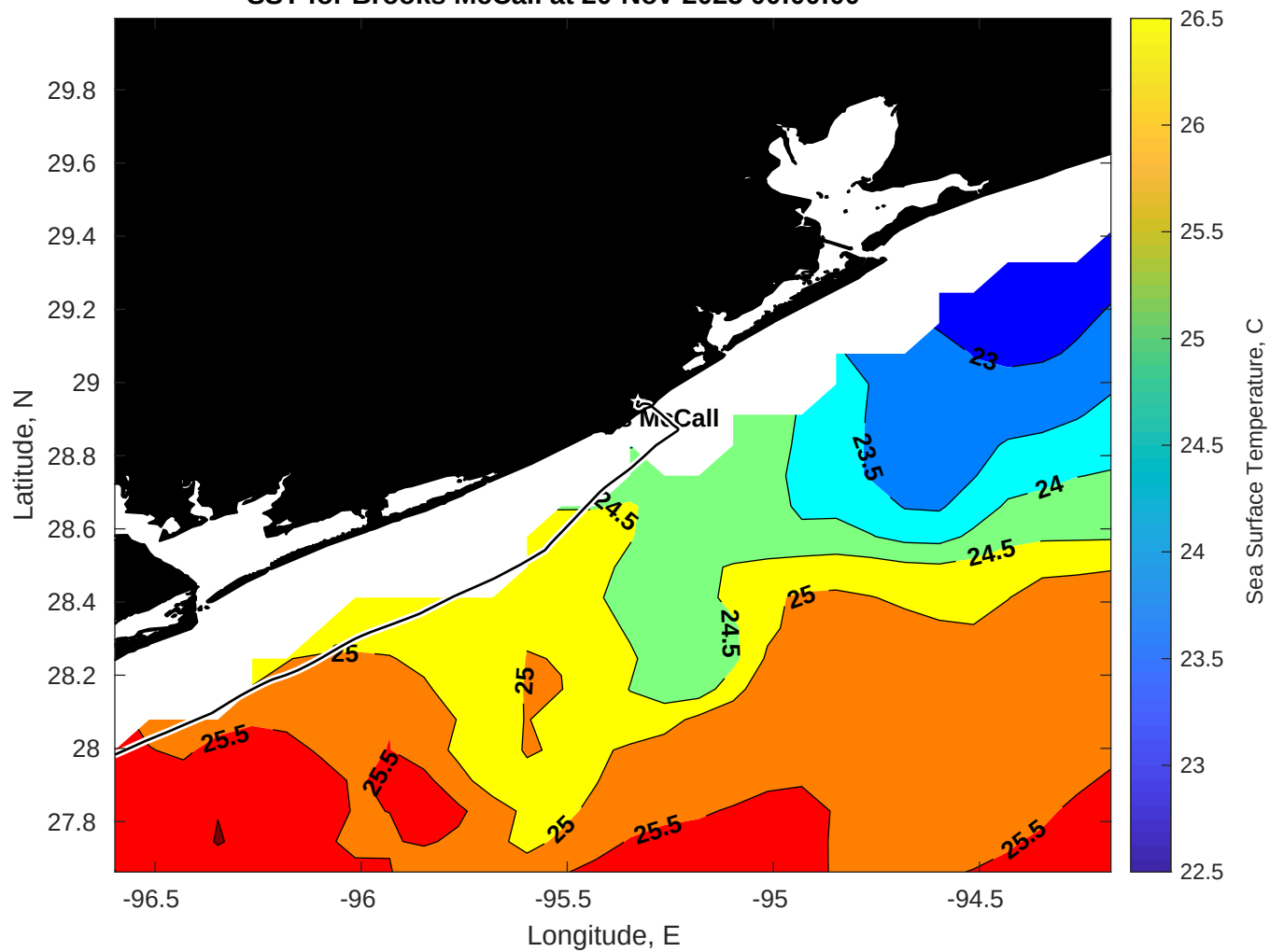
SST for Brooks McCall at 20-Nov-2025 00:00:00
