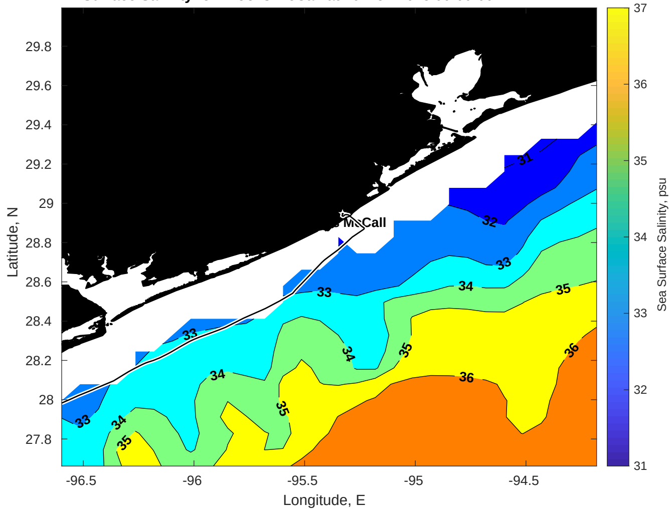
Surface Salinity for Brooks McCall at 20-Nov-2025 00:00:00
