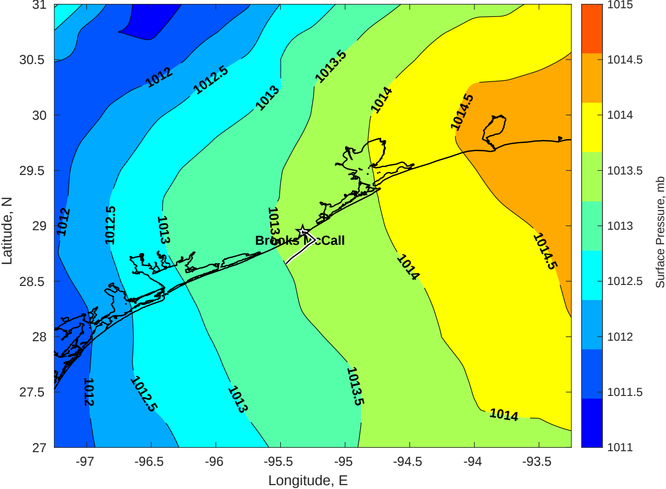
Surface Pressure (mb) for Brooks McCall at 21-Nov-2025 00:00:00
