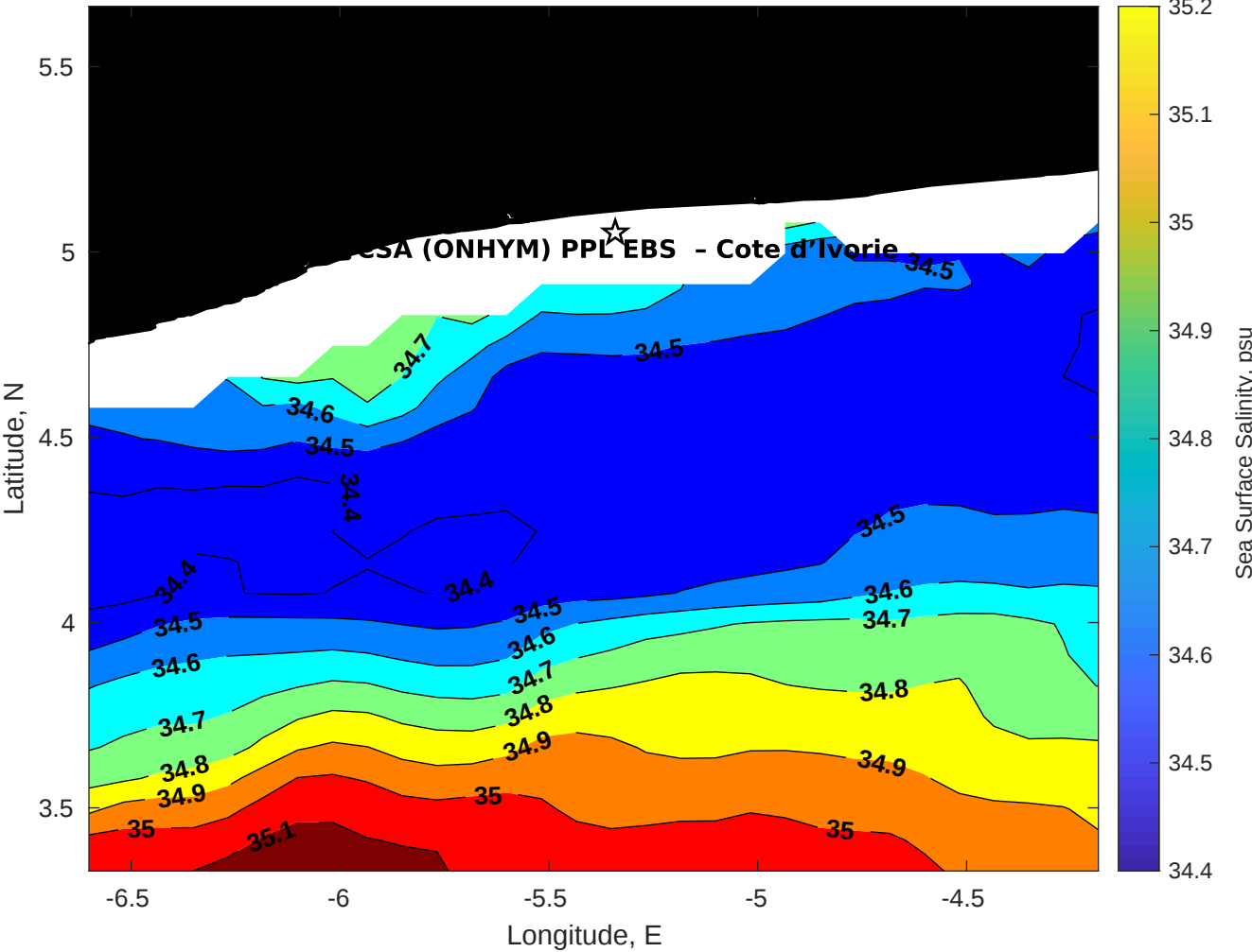
Surface Salinity for CSA (ONHYM) PPL EBS - Cote d'Ivoire at 20-Nov-2025 00:00:00
