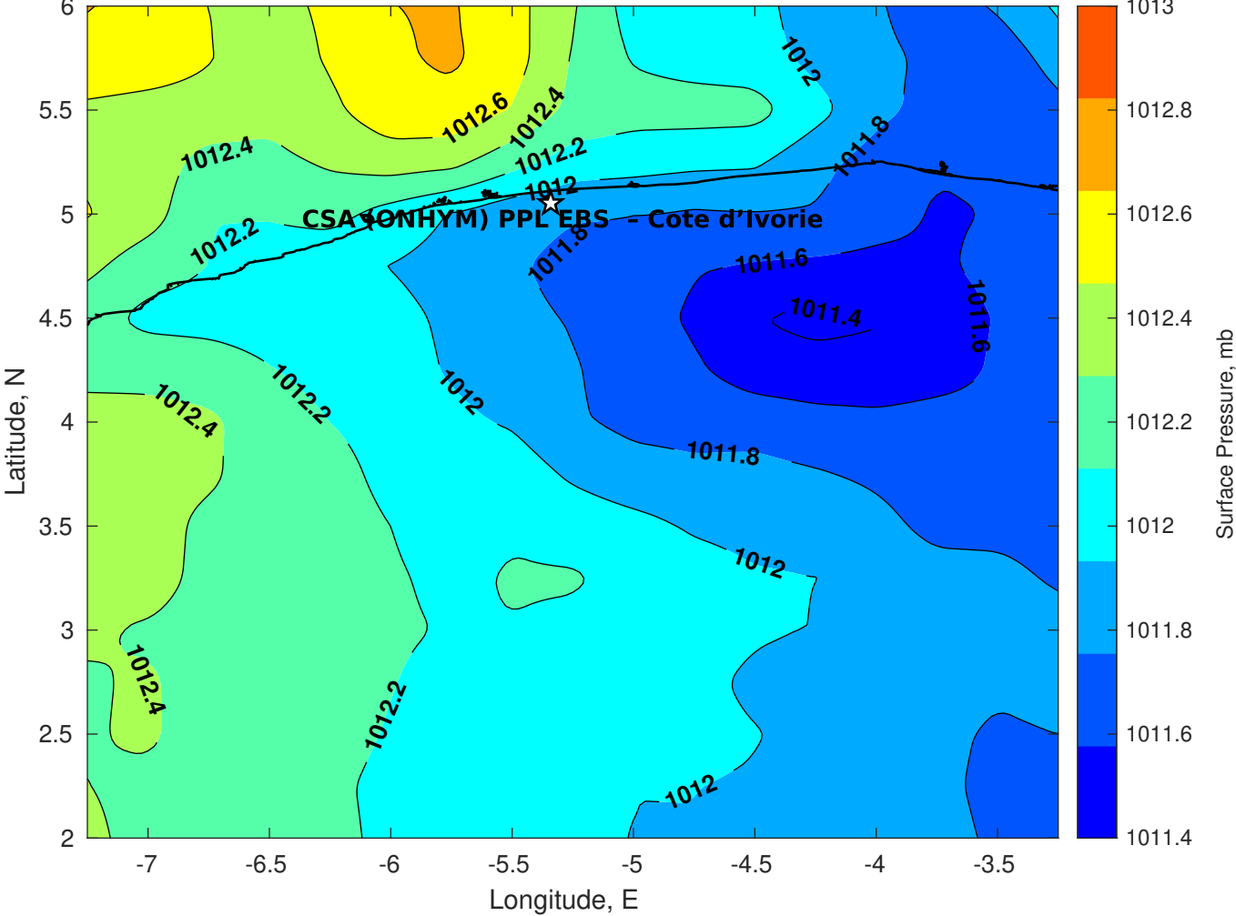
Surface Pressure (mb) for CSA (ONHYM) PPL EBS - Cote d'Ivoire at 21-Nov-2025 00:00:00
