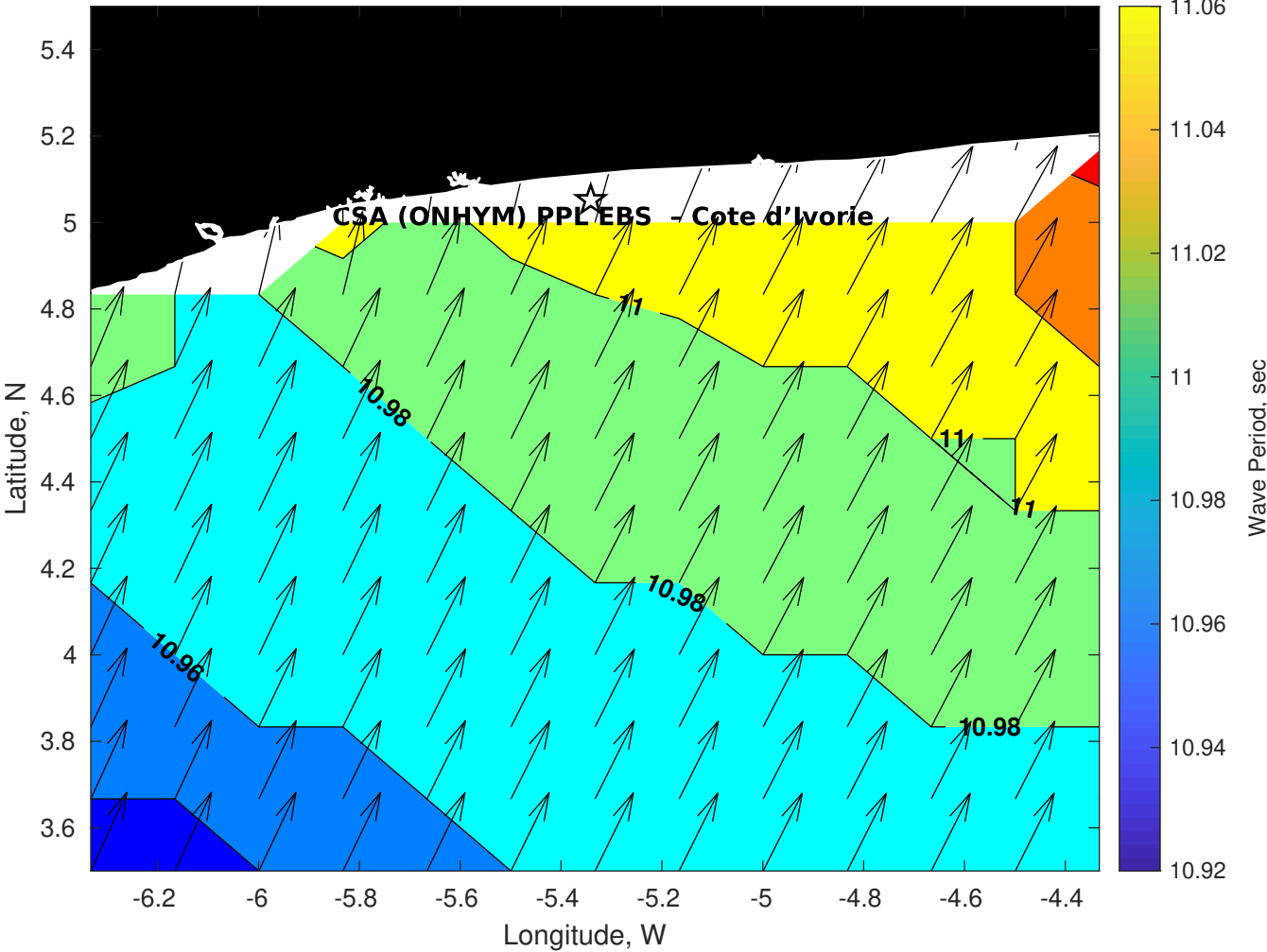
Wave Period (sec) for CSA (ONHYM) PPL EBS - Cote d'Ivoire at 19-Nov-2025 21:00:00
