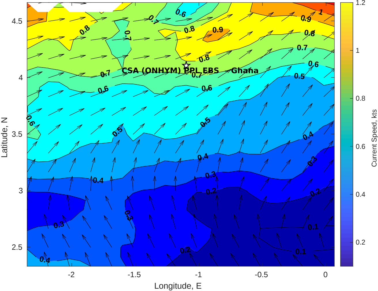
Surface Currents for CSA (ONHYM) PPL EBS - Ghana at 20-Nov-2025 00:00:00
