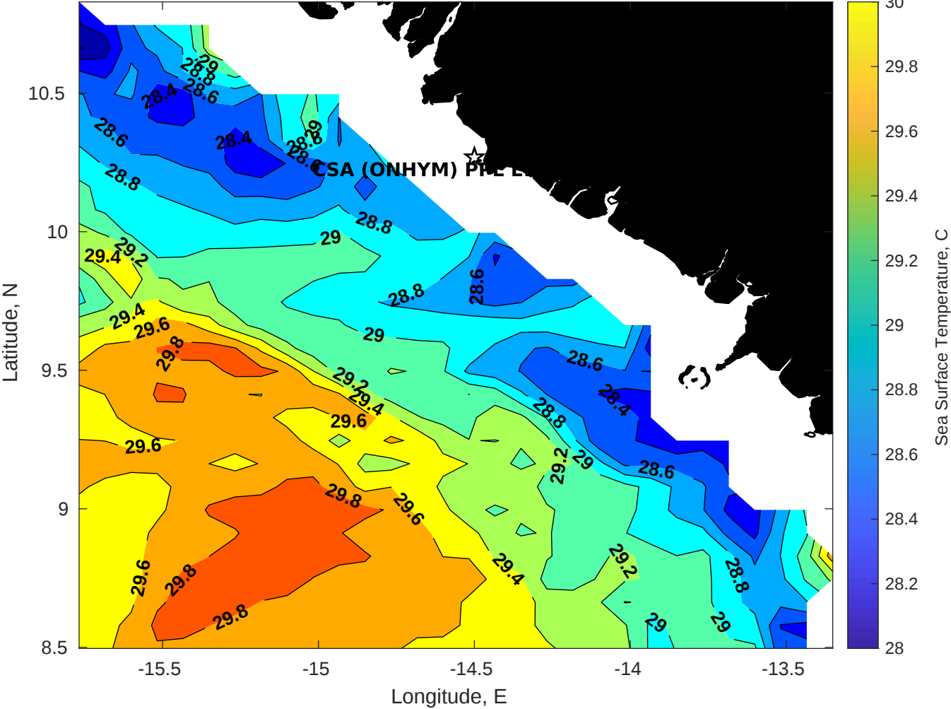
SST for CSA (ONHYM) PPL EBS - Guinea at 20-Nov-2025 00:00:00
