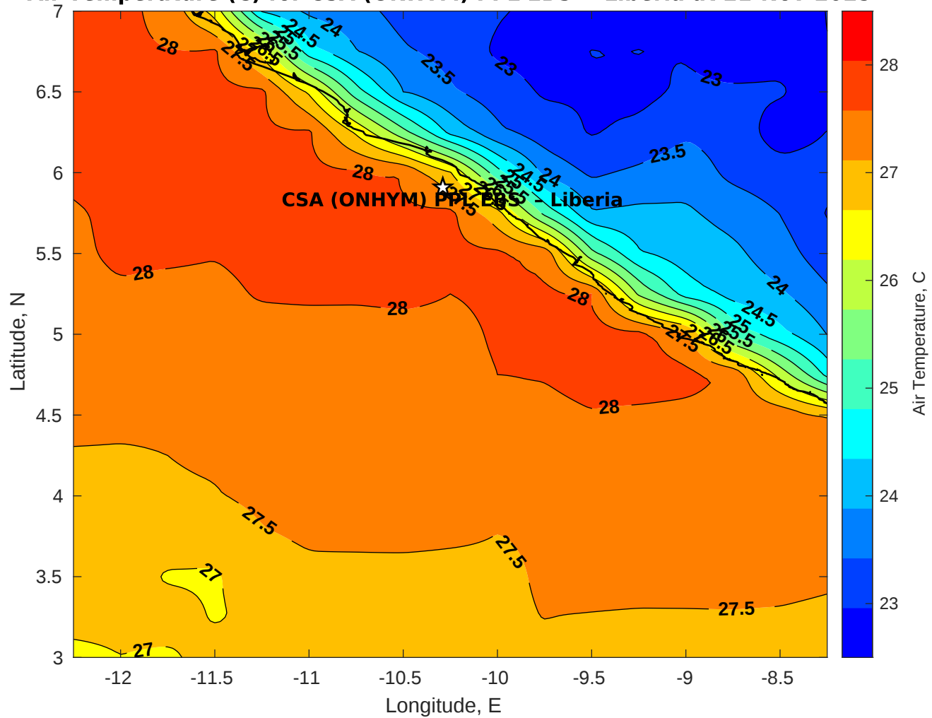
Air Temperature (C) for CSA (ONHYM) PPL EBS - Liberia at 21-Nov-2025
