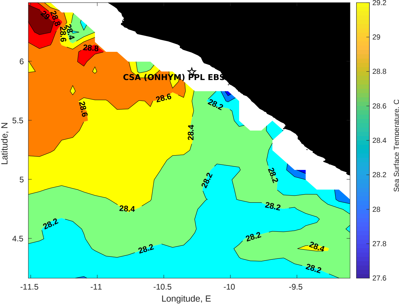
SST for CSA (ONHYM) PPL EBS - Liberia at 20-Nov-2025 00:00:00
