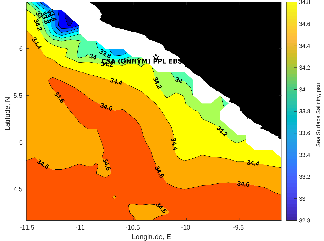
Surface Salinity for CSA (ONHYM) PPL EBS - Liberia at 20-Nov-2025 00:00:00
