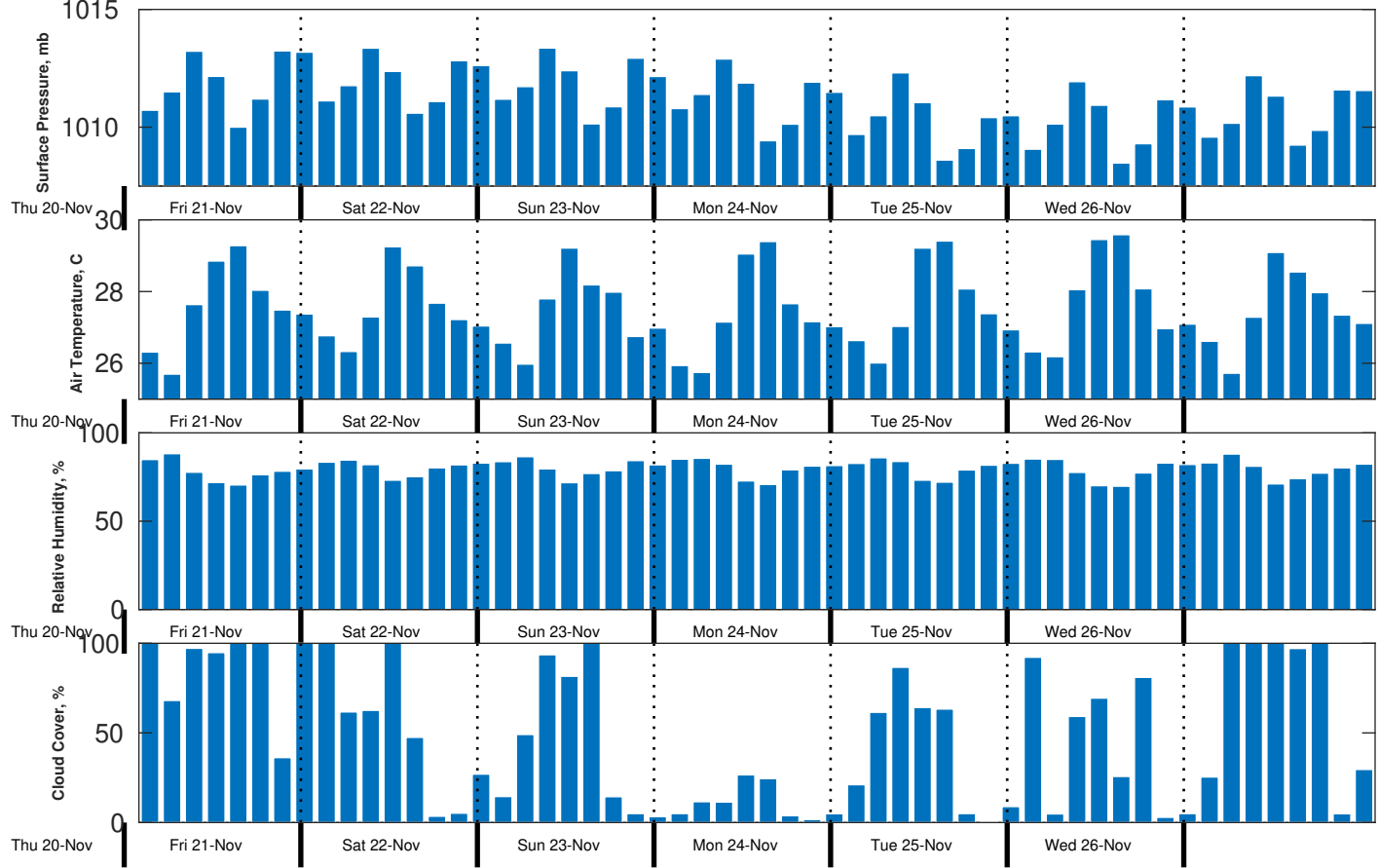
Met Forecast for CSA (ONHYM) PPL EBS - Liberia from 21-Nov-2025 00:00:00 to 28-Nov-2025 00:00:00
