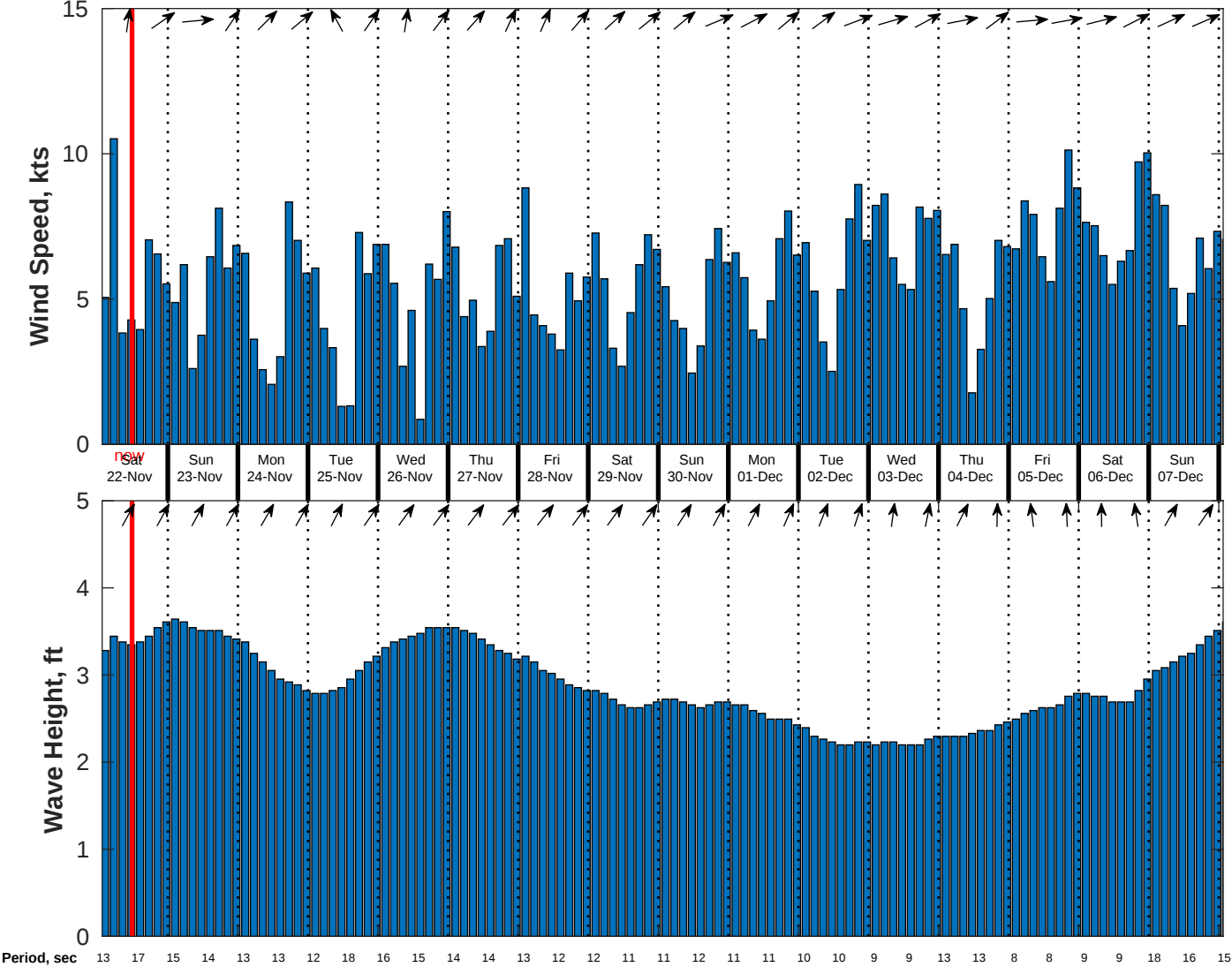
Wind & Wave Forecast for CSA (ONHYM) PPL EBS - Liberia from 21-Nov-2025 01:00:00 to 07-Dec-2025 01:00:00
