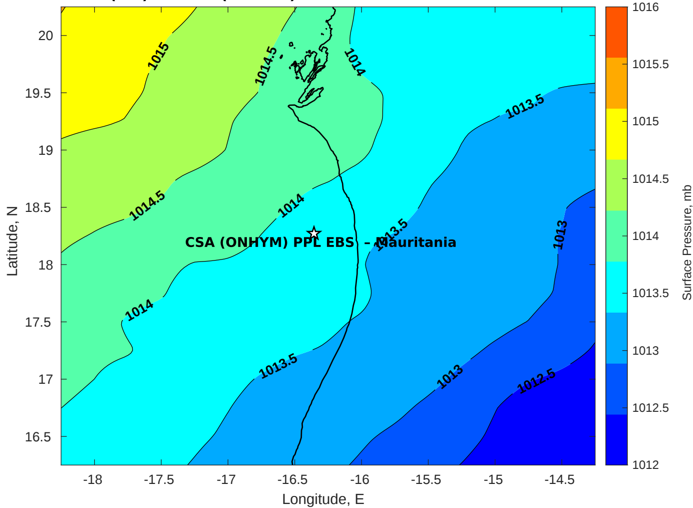
Surface Pressure (mb) for CSA (ONHYM) PPL EBS - Mauritania at 21-Nov-2025 00:00:00
