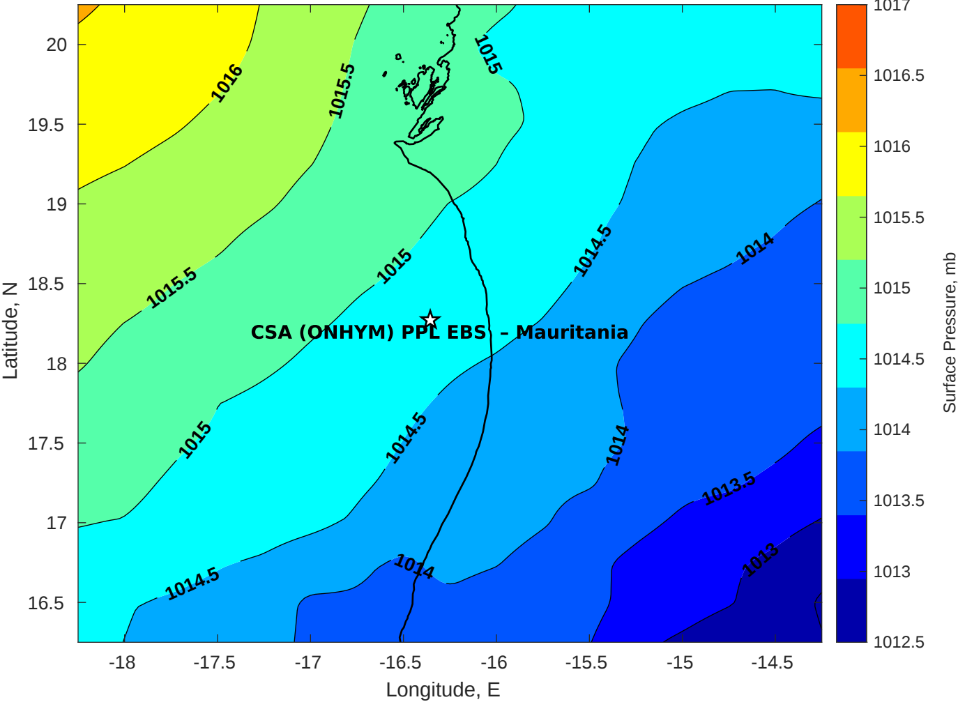
Surface Pressure (mb) for CSA (ONHYM) PPL EBS - Mauritania at 22-Nov-2025 00:00:00
