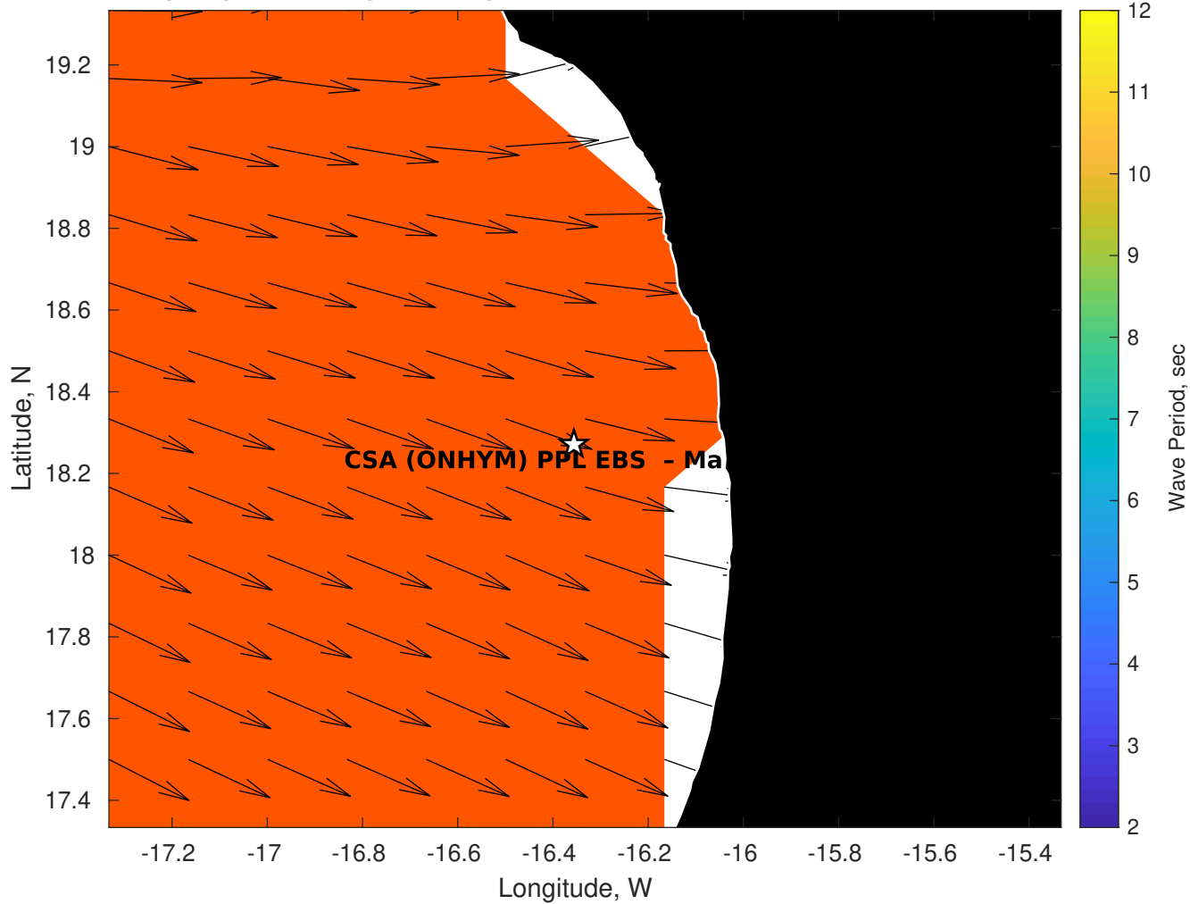
Wave Period (sec) for CSA (ONHYM) PPL EBS - Mauritania at 19-Nov-2025 21:00:00
