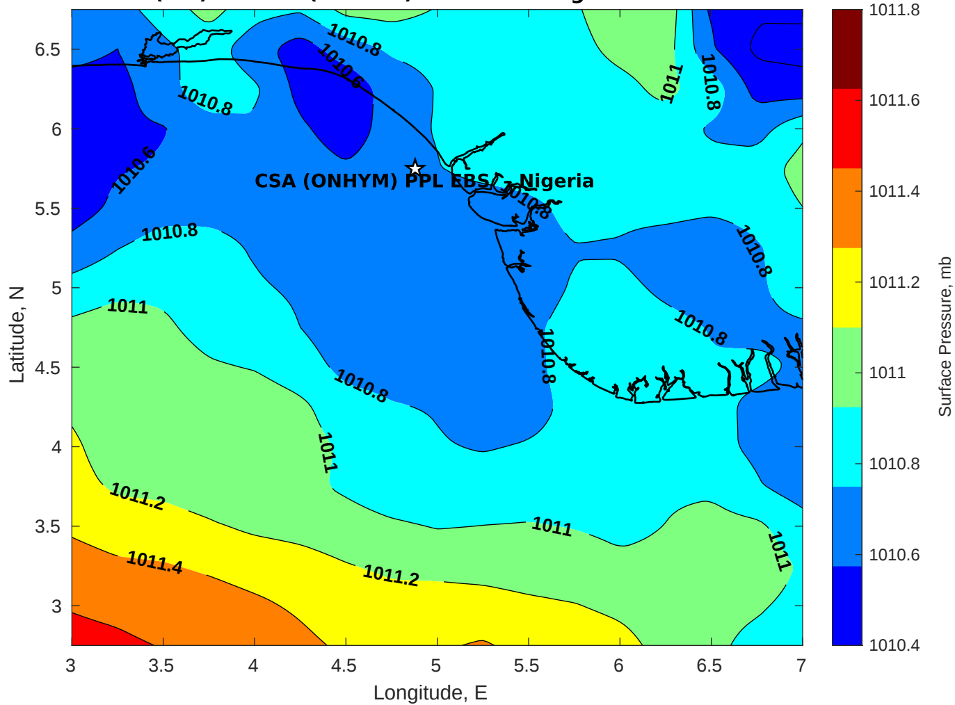
Surface Pressure (mb) for CSA (ONHYM) PPL EBS - Nigeria at 22-Nov-2025 00:00:00
