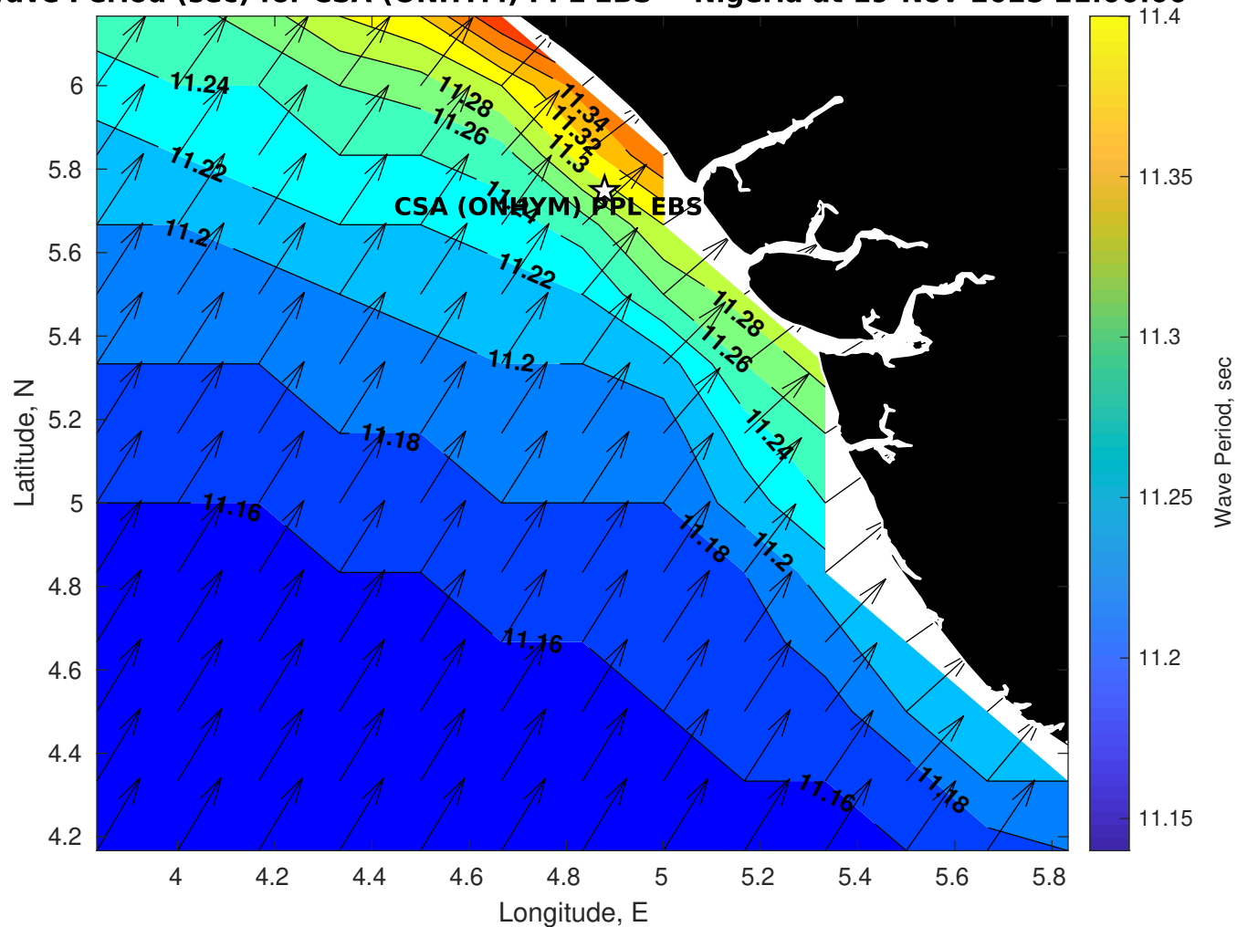
Wave Period (sec) for CSA (ONHYM) PPL EBS - Nigeria at 19-Nov-2025 21:00:00
