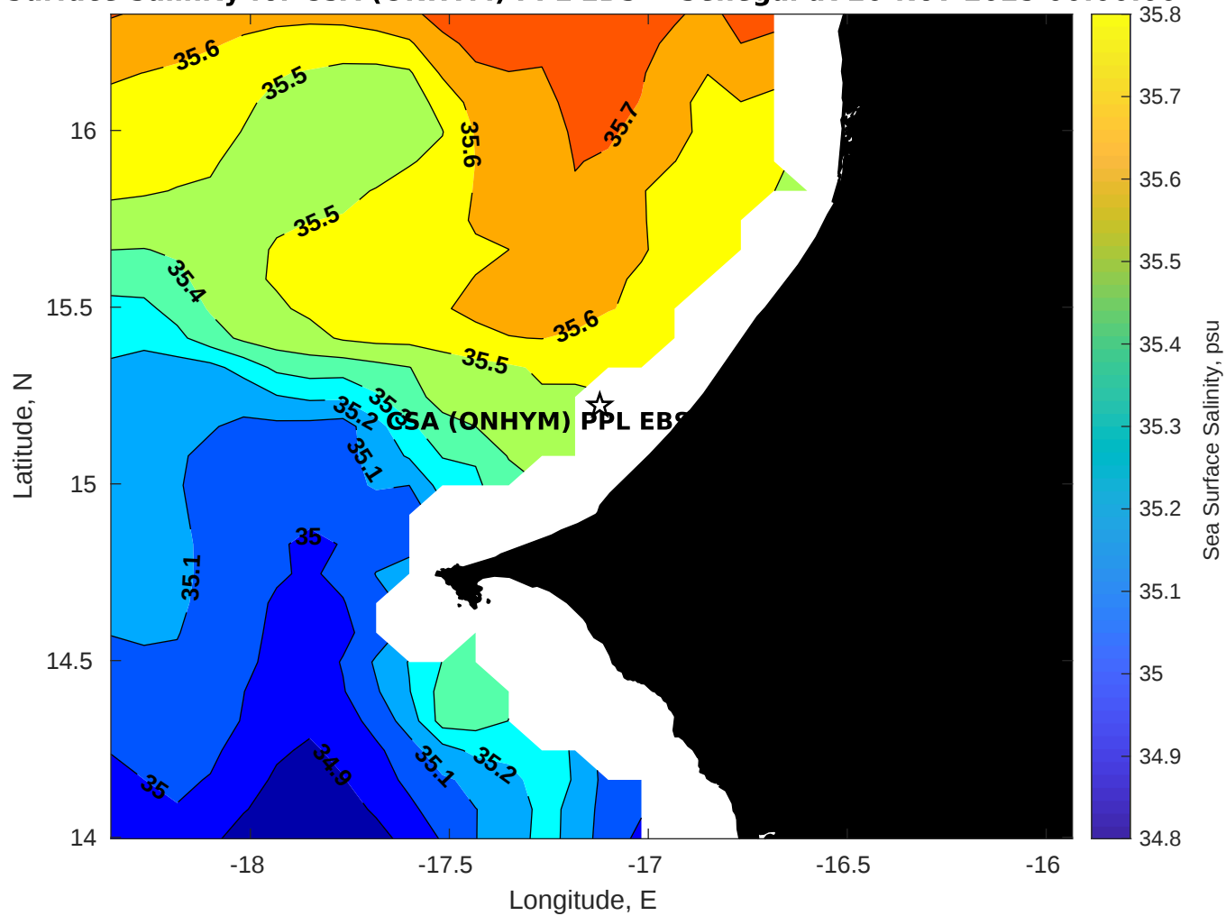
Surface Salinity for CSA (ONHYM) PPL EBS - Senegal at 20-Nov-2025 00:00:00
