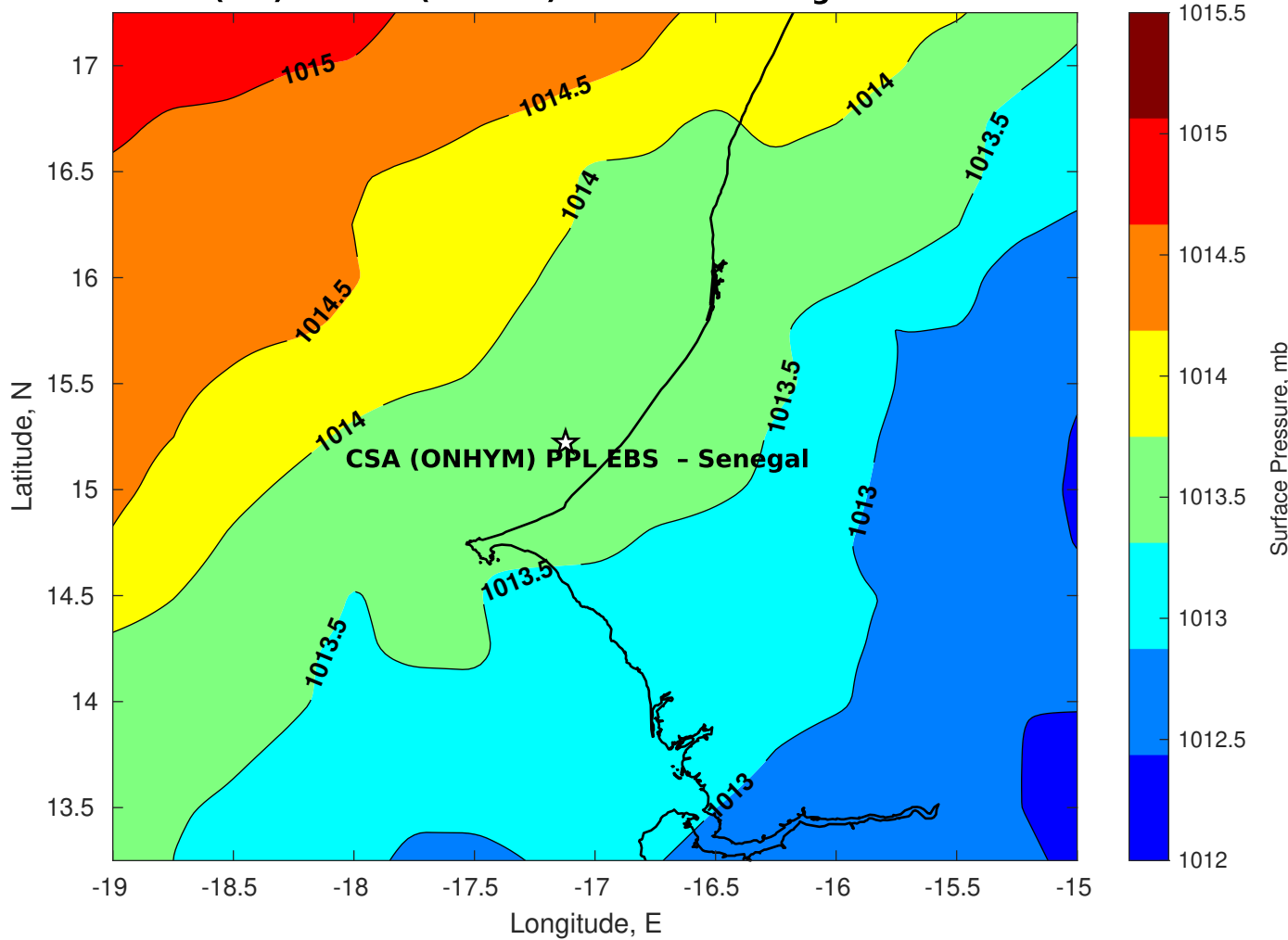
Surface Pressure (mb) for CSA (ONHYM) PPL EBS - Senegal at 22-Nov-2025 00:00:00
