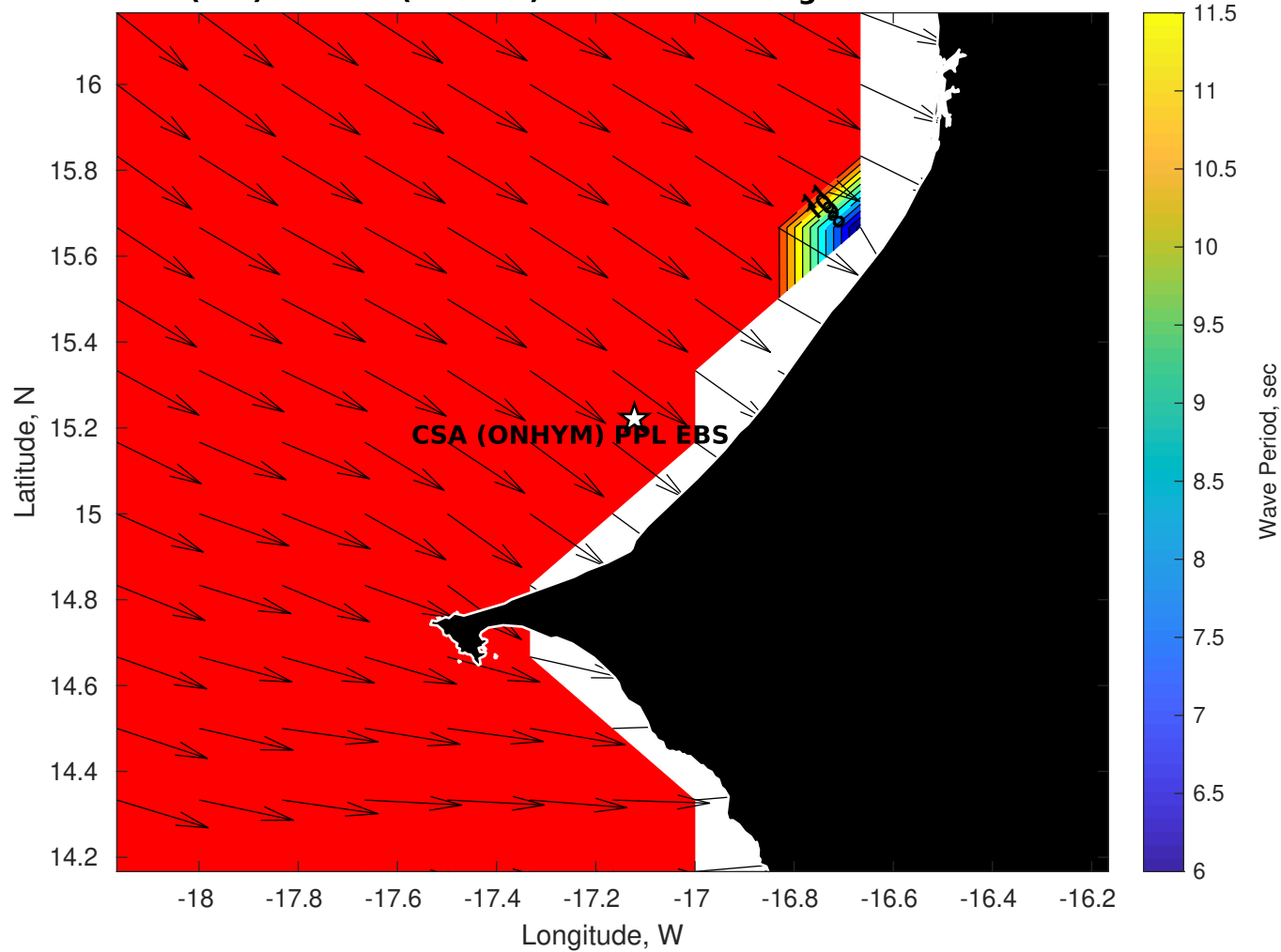
Wave Period (sec) for CSA (ONHYM) PPL EBS - Senegal at 19-Nov-2025 21:00:00
