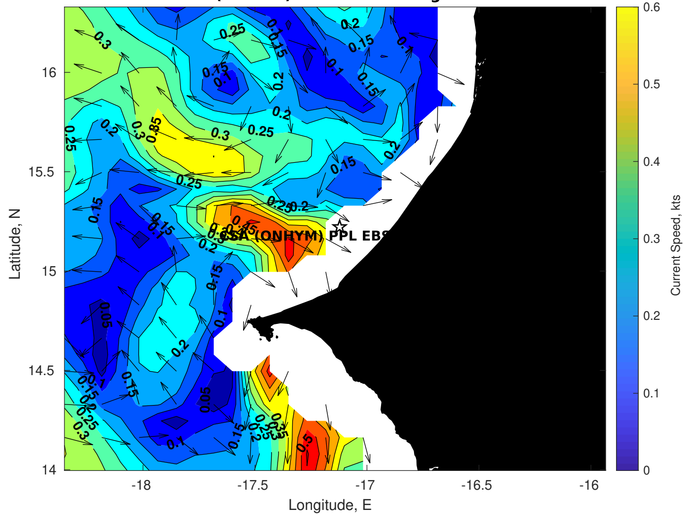
Surface Currents for CSA (ONHYM) PPL EBS - Senegal at 20-Nov-2025 00:00:00
