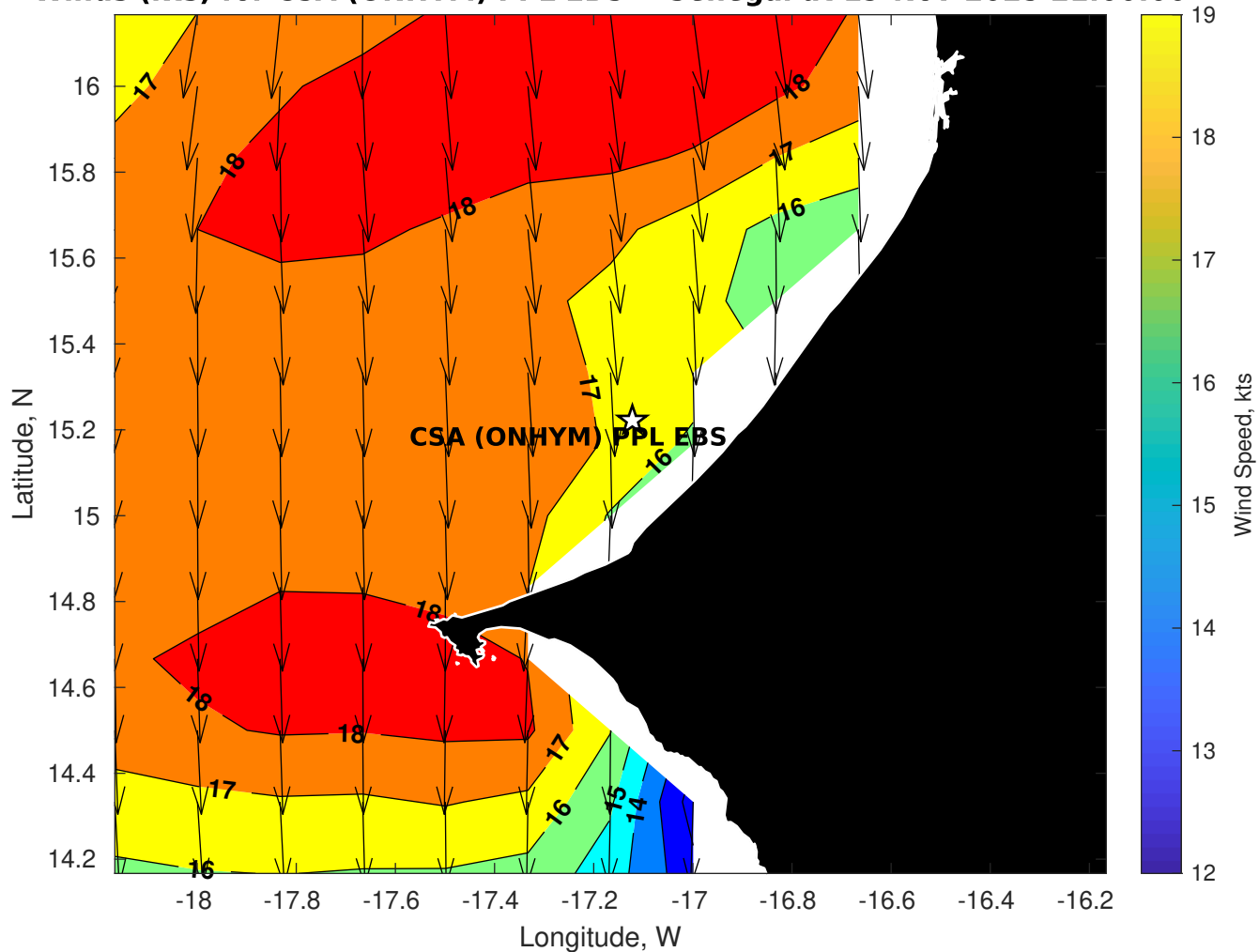
Winds (kts) for CSA (ONHYM) PPL EBS - Senegal at 19-Nov-2025 21:00:00
