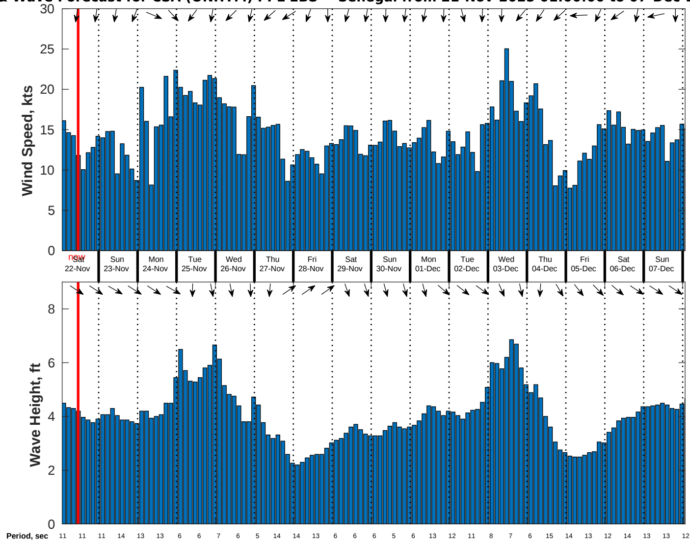
Wind & Wave Forecast for CSA (ONHYM) PPL EBS - Senegal from 21-Nov-2025 01:00:00 to 07-Dec-2025 01:00:00
