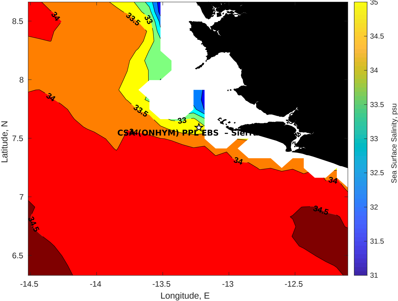
Surface Salinity for CSA (ONHYM) PPL EBS - Sierra Leone at 20-Nov-2025 00:00:00
