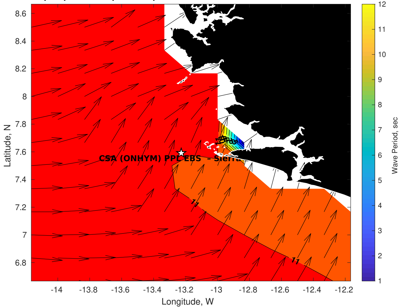
Wave Period (sec) for CSA (ONHYM) PPL EBS - Sierra Leone at 19-Nov-2025 21:00:00
