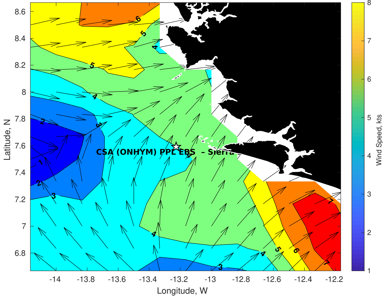
Winds (kts) for CSA (ONHYM) PPL EBS - Sierra Leone at 19-Nov-2025 21:00:00
