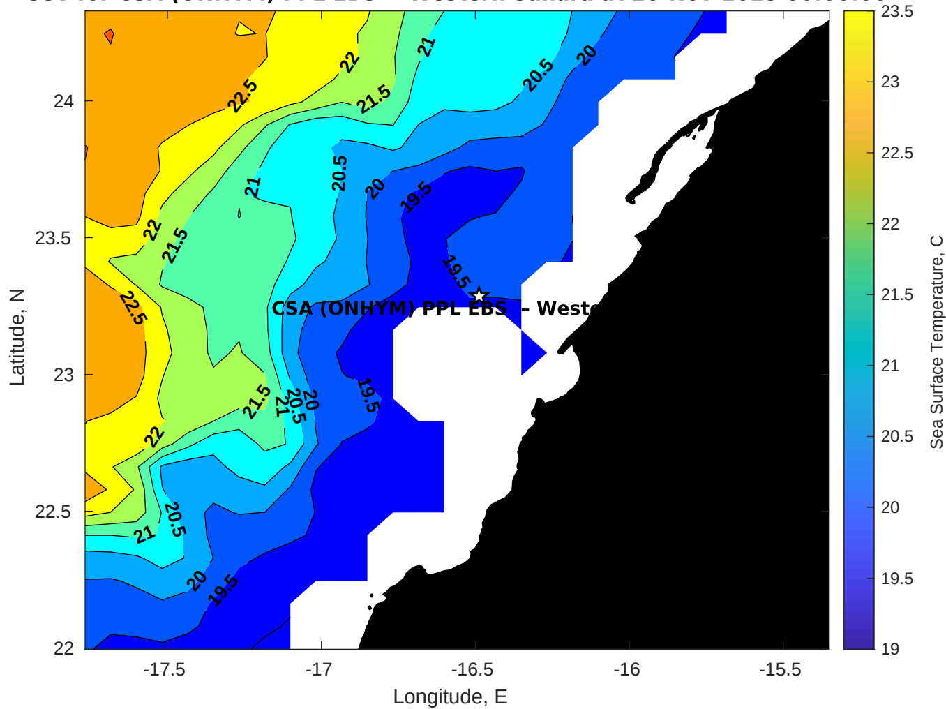
SST for CSA (ONHYM) PPL EBS - Western Sahara at 20-Nov-2025 00:00:00
