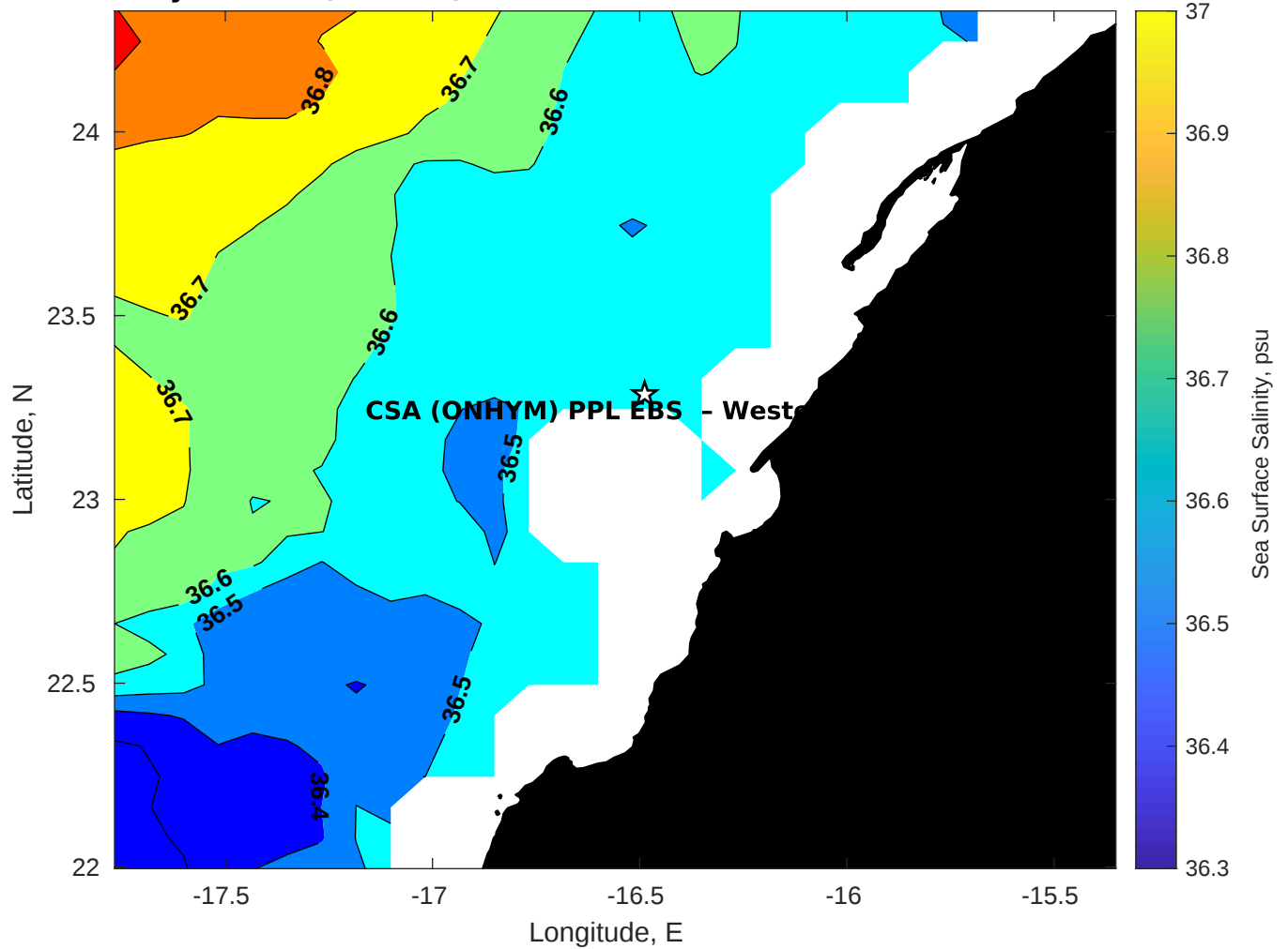
Surface Salinity for CSA (ONHYM) PPL EBS - Western Sahara at 20-Nov-2025 00:00:00
