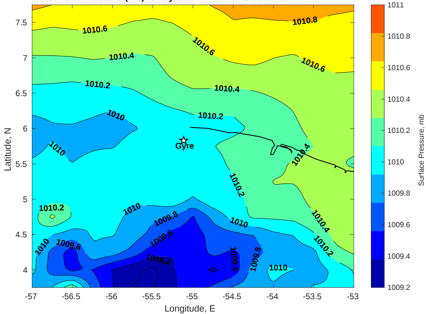
Surface Pressure (mb) for Gyre at 21-Nov-2025 00:00:00
