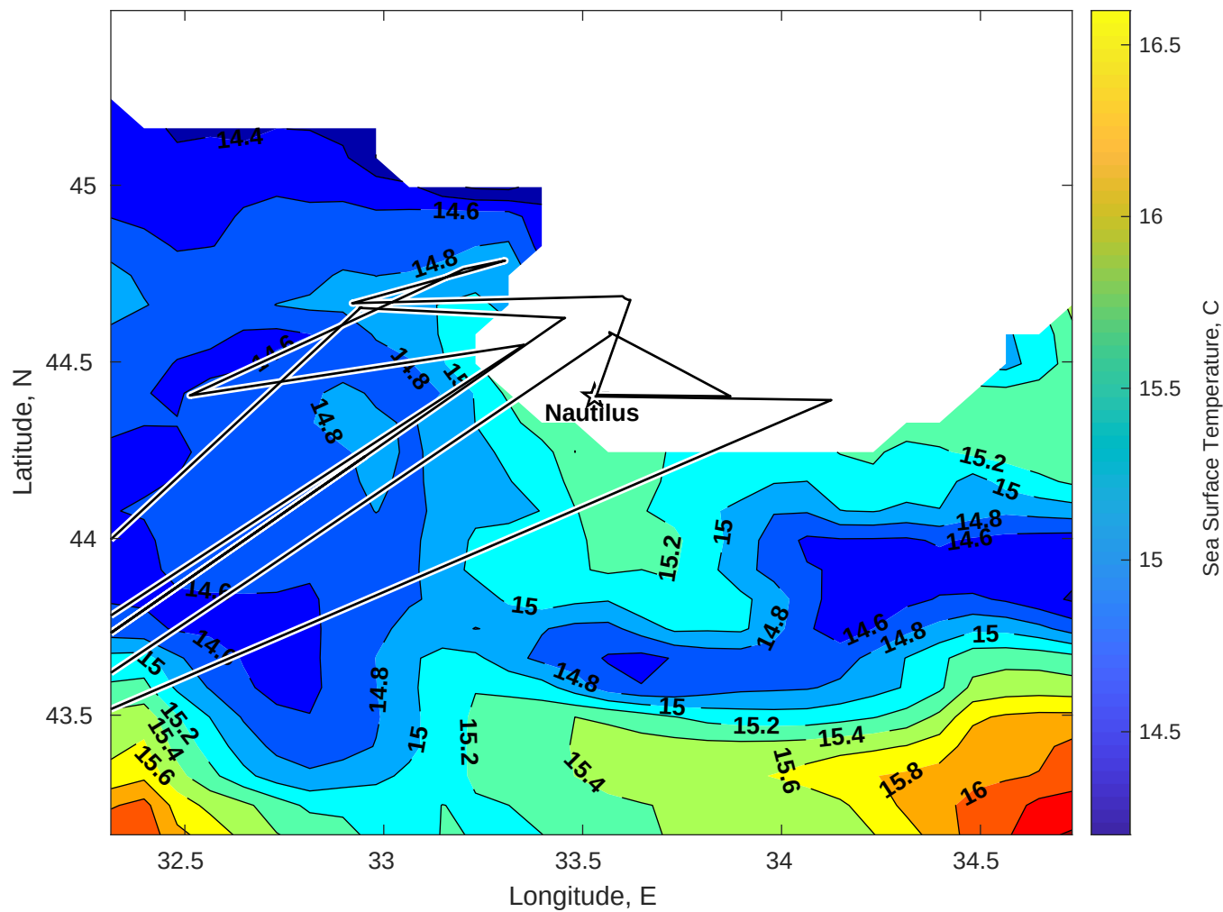
SST for Nautilus at 20-Nov-2025 00:00:00
