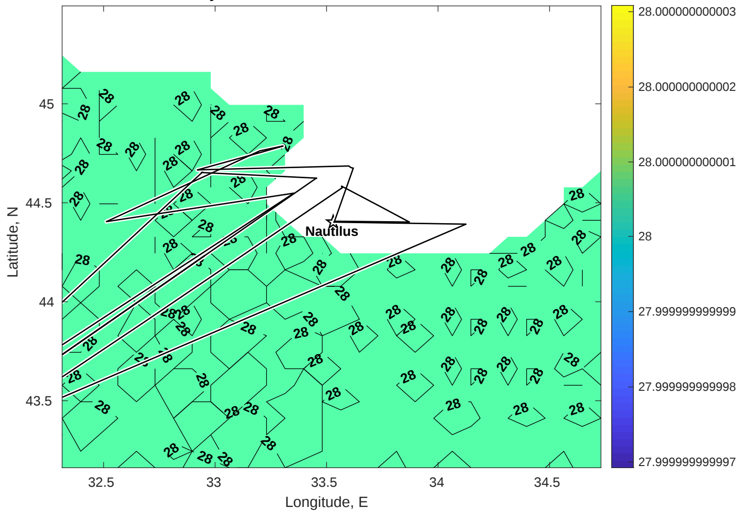
Surface Salinity for Nautilus at 20-Nov-2025 00:00:00
