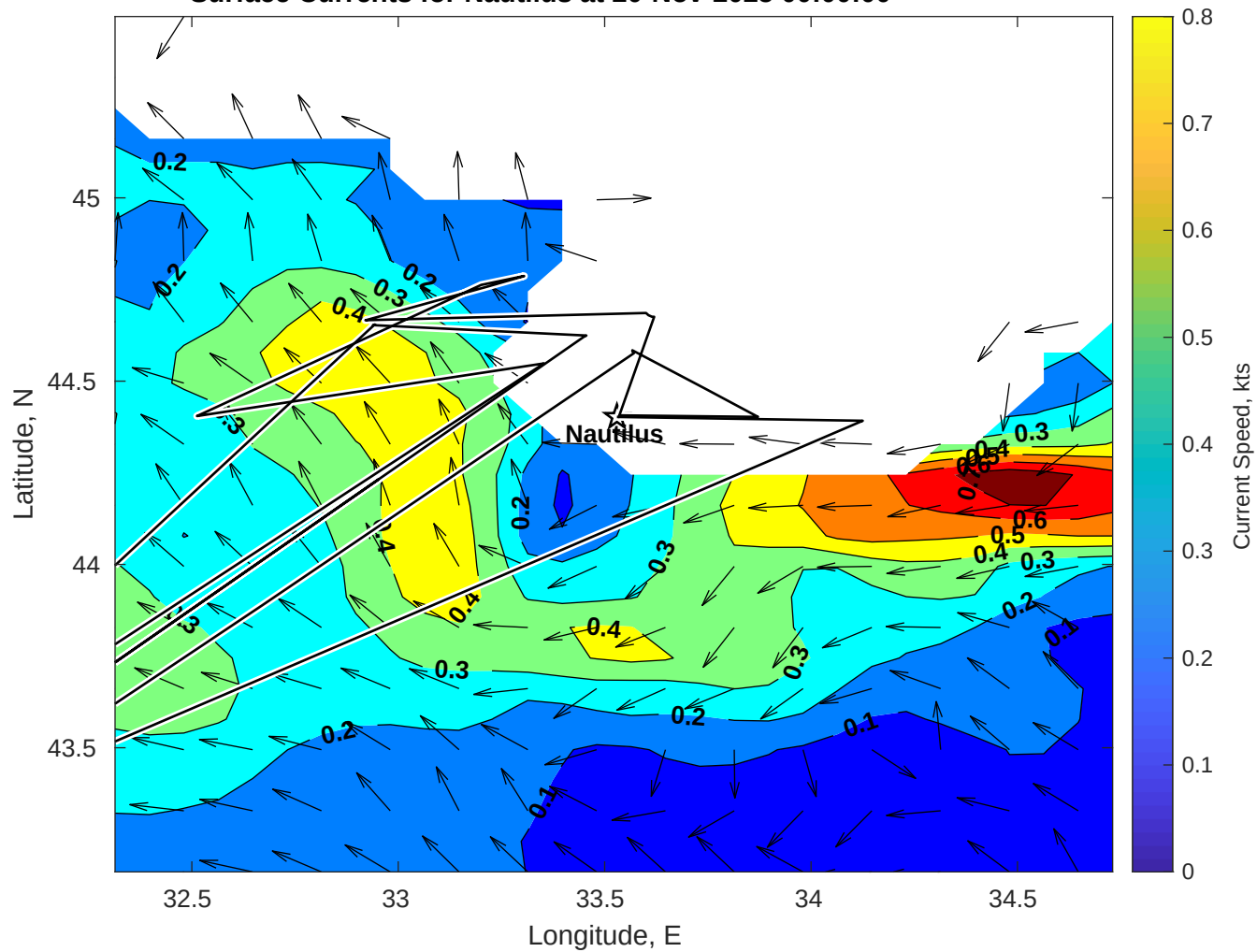
Surface Currents for Nautilus at 20-Nov-2025 00:00:00
