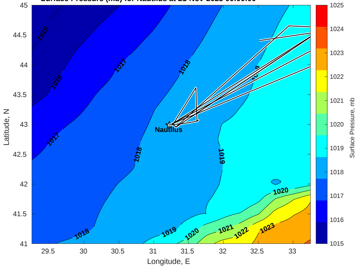
Surface Pressure (mb) for Nautilus at 21-Nov-2025 00:00:00
