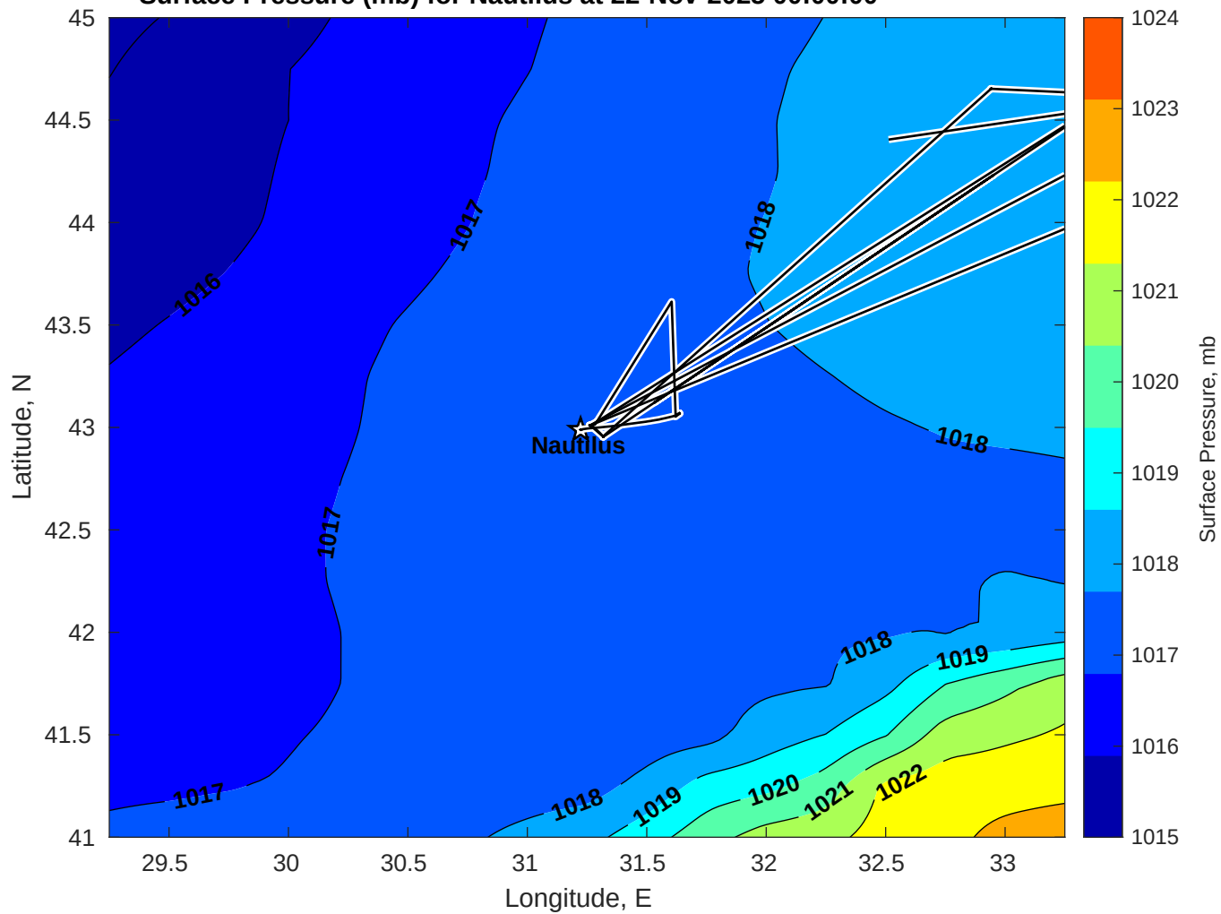
Surface Pressure (mb) for Nautilus at 22-Nov-2025 00:00:00
