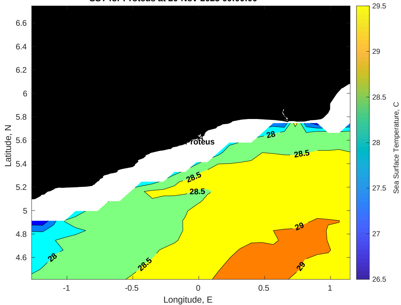
SST for Proteus at 20-Nov-2025 00:00:00
