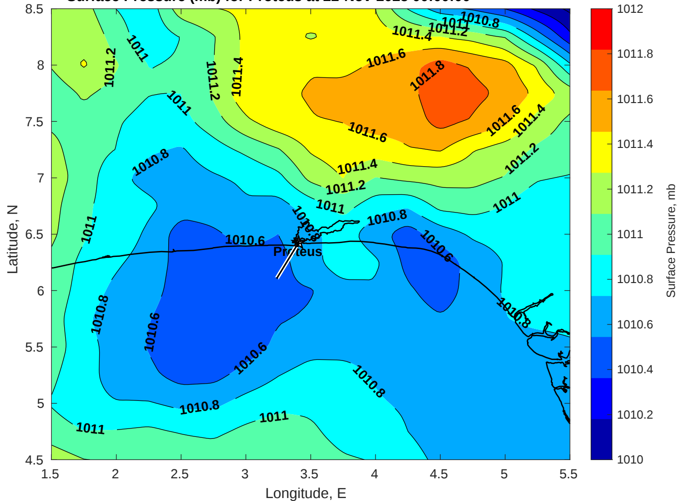
Surface Pressure (mb) for Proteus at 22-Nov-2025 00:00:00
