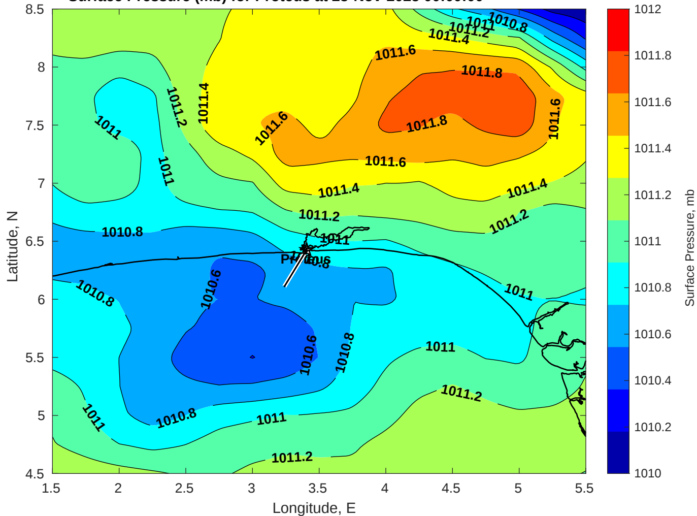
Surface Pressure (mb) for Proteus at 23-Nov-2025 00:00:00
