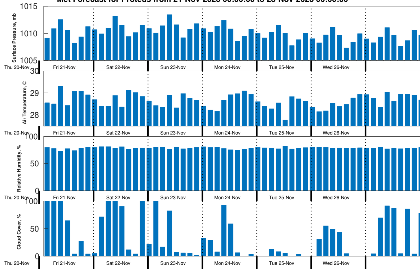
Met Forecast for Proteus from 21-Nov-2025 00:00:00 to 28-Nov-2025 00:00:00
