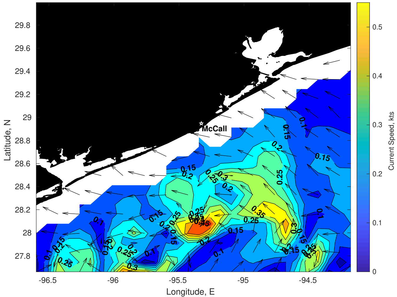
Surface Currents for Brooks McCall at 21-Nov-2025 00:00:00
