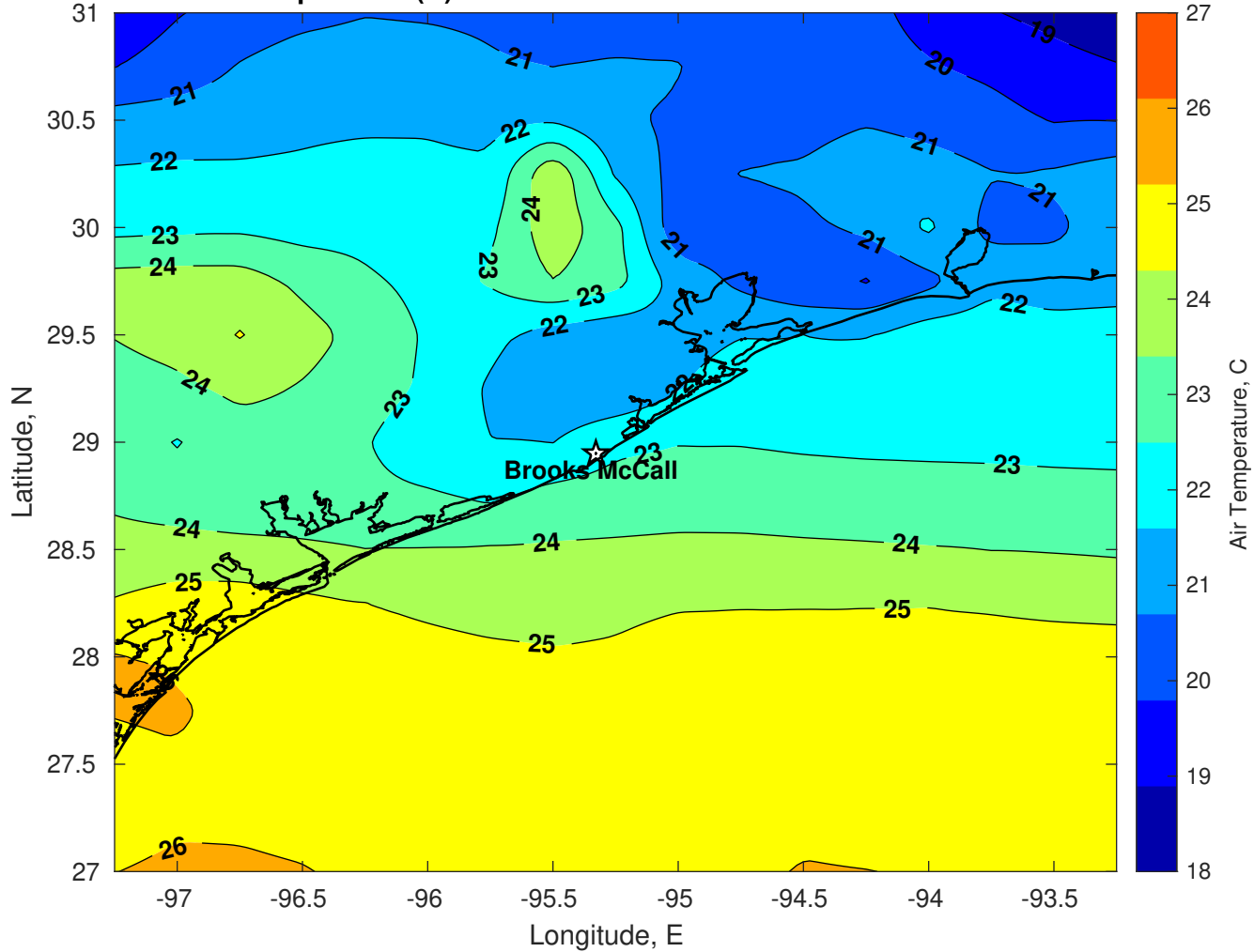
Air Temperature (C) for Brooks McCall at 22-Nov-2025
