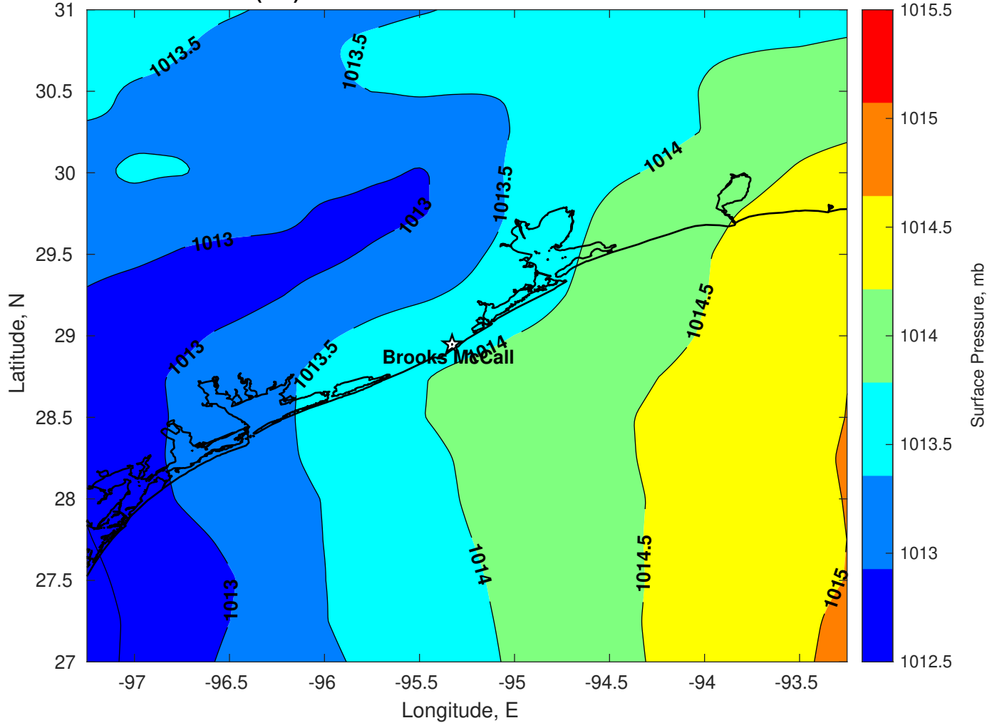
Surface Pressure (mb) for Brooks McCall at 22-Nov-2025 00:00:00
