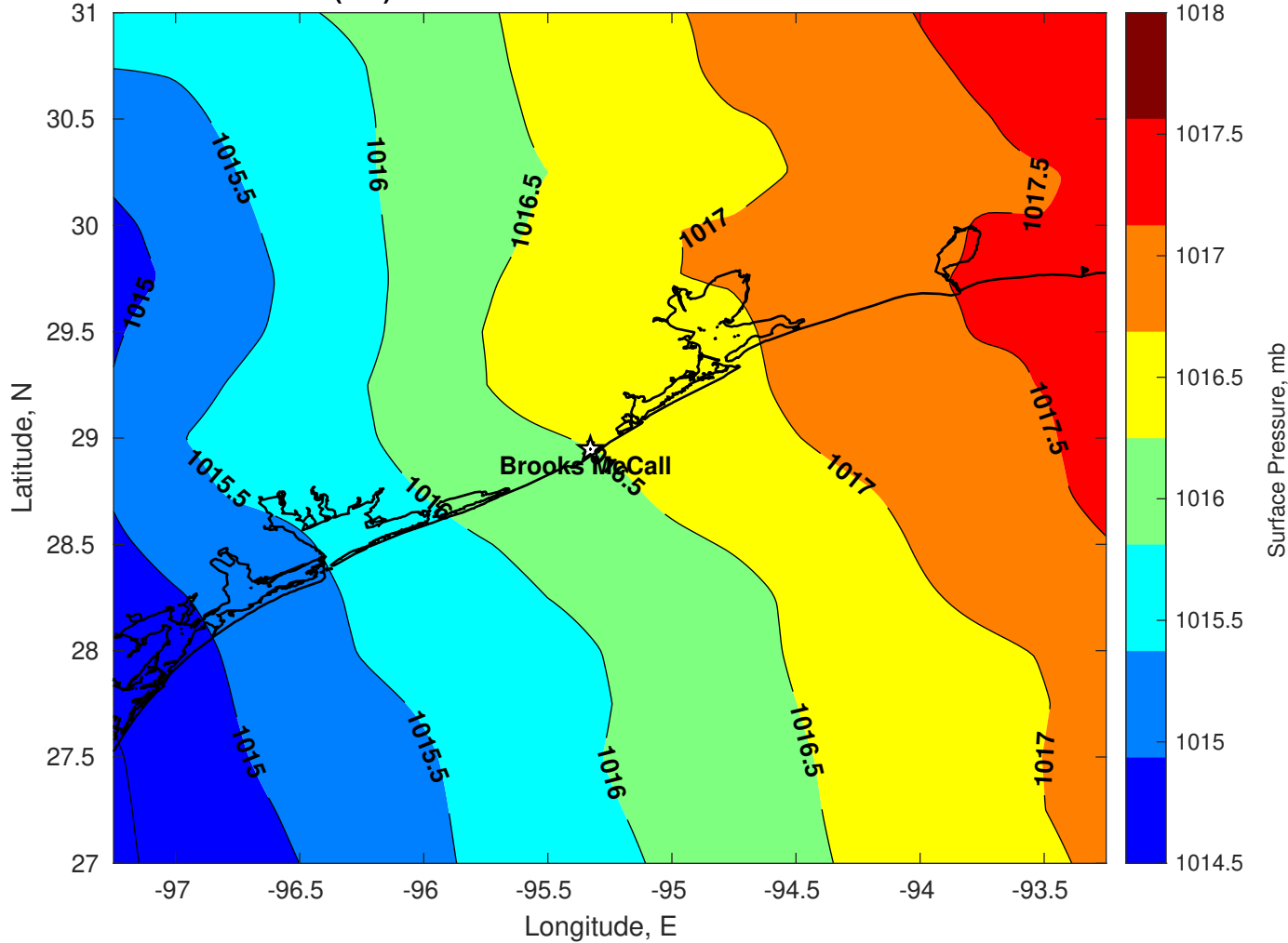
Surface Pressure (mb) for Brooks McCall at 24-Nov-2025 00:00:00
