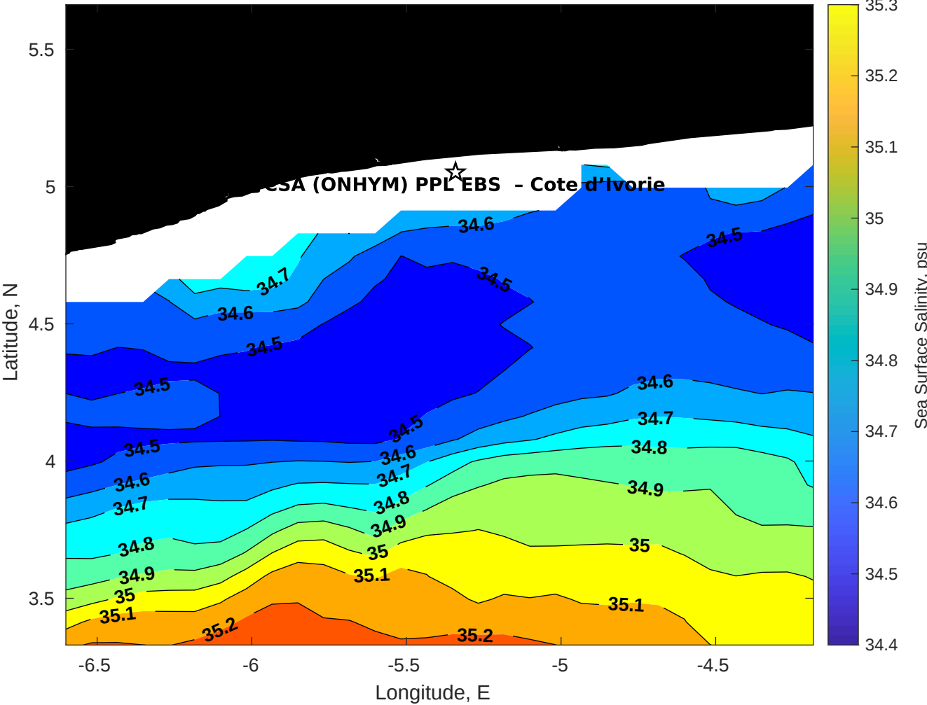
Surface Salinity for CSA (ONHYM) PPL EBS - Cote d'Ivoire at 21-Nov-2025 00:00:00
